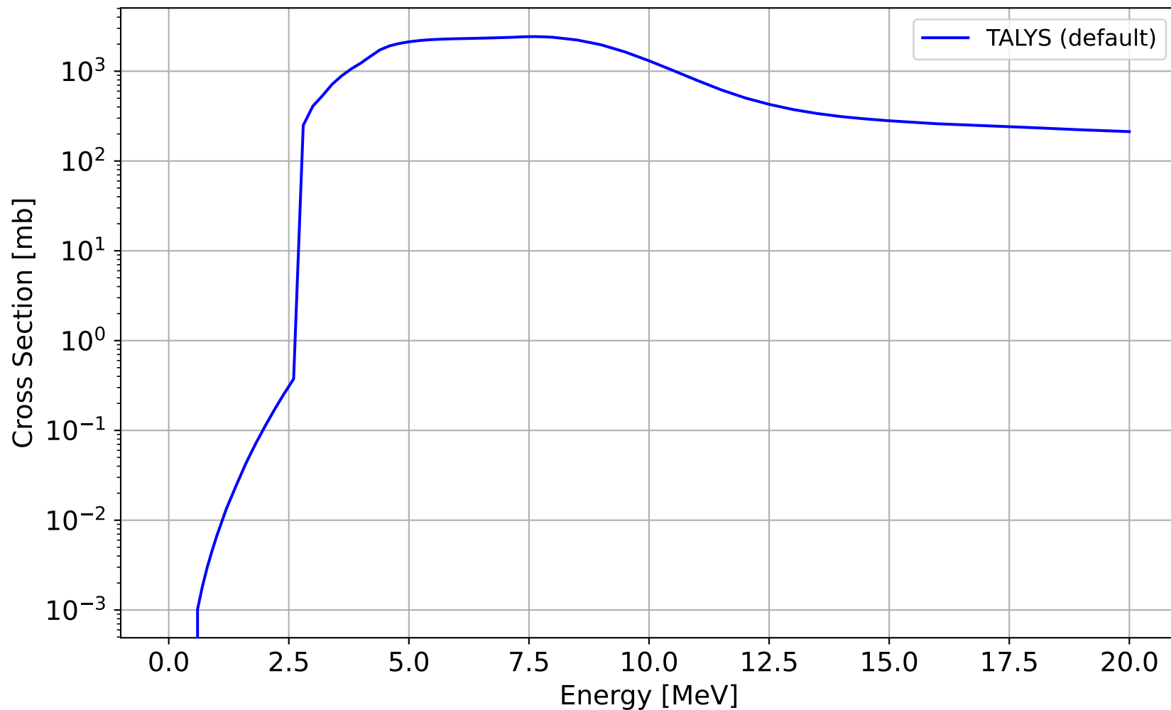
^{208}\text{Pb}(n,n')^{208}\text{Pb} cross section from TALYS
