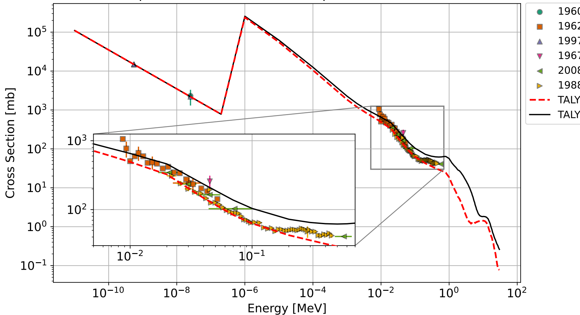
^{119}\text{Sn}(n,\gamma)^{120}\text{Sn} Cross Sections Comparison with EXFOR Data
