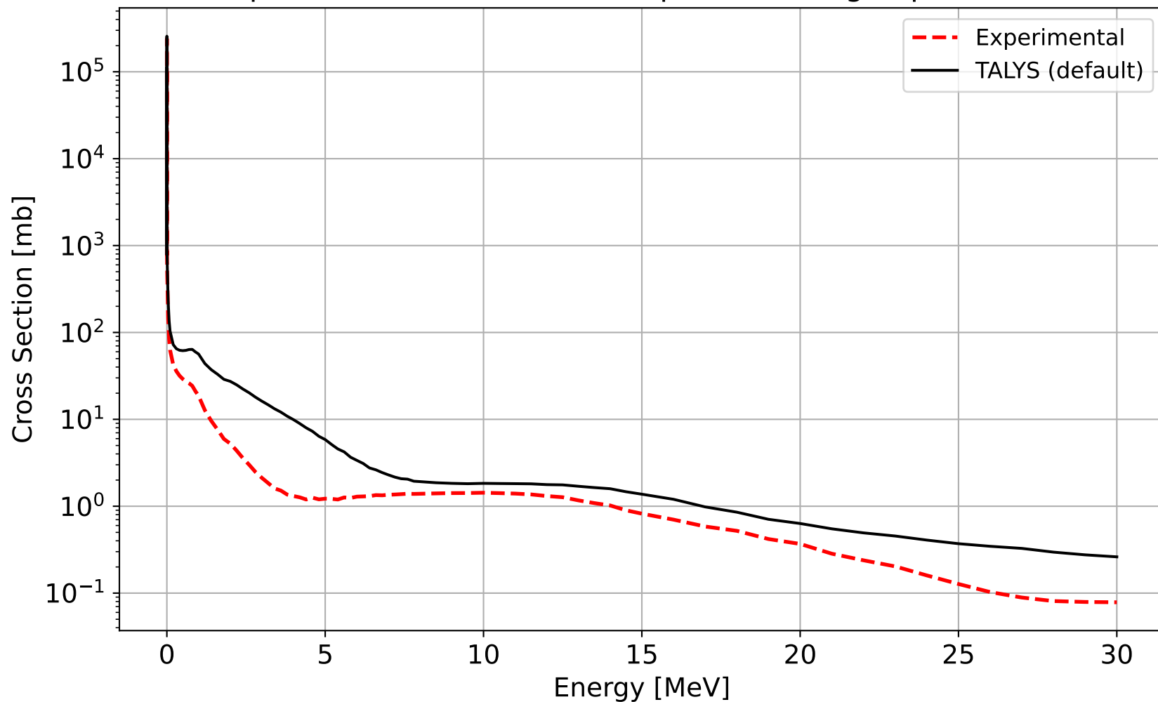
^{119}\text{Sn}(n,\gamma)^{120}\text{Sn} Cross Sections Comparison Using Experimental GSFs
