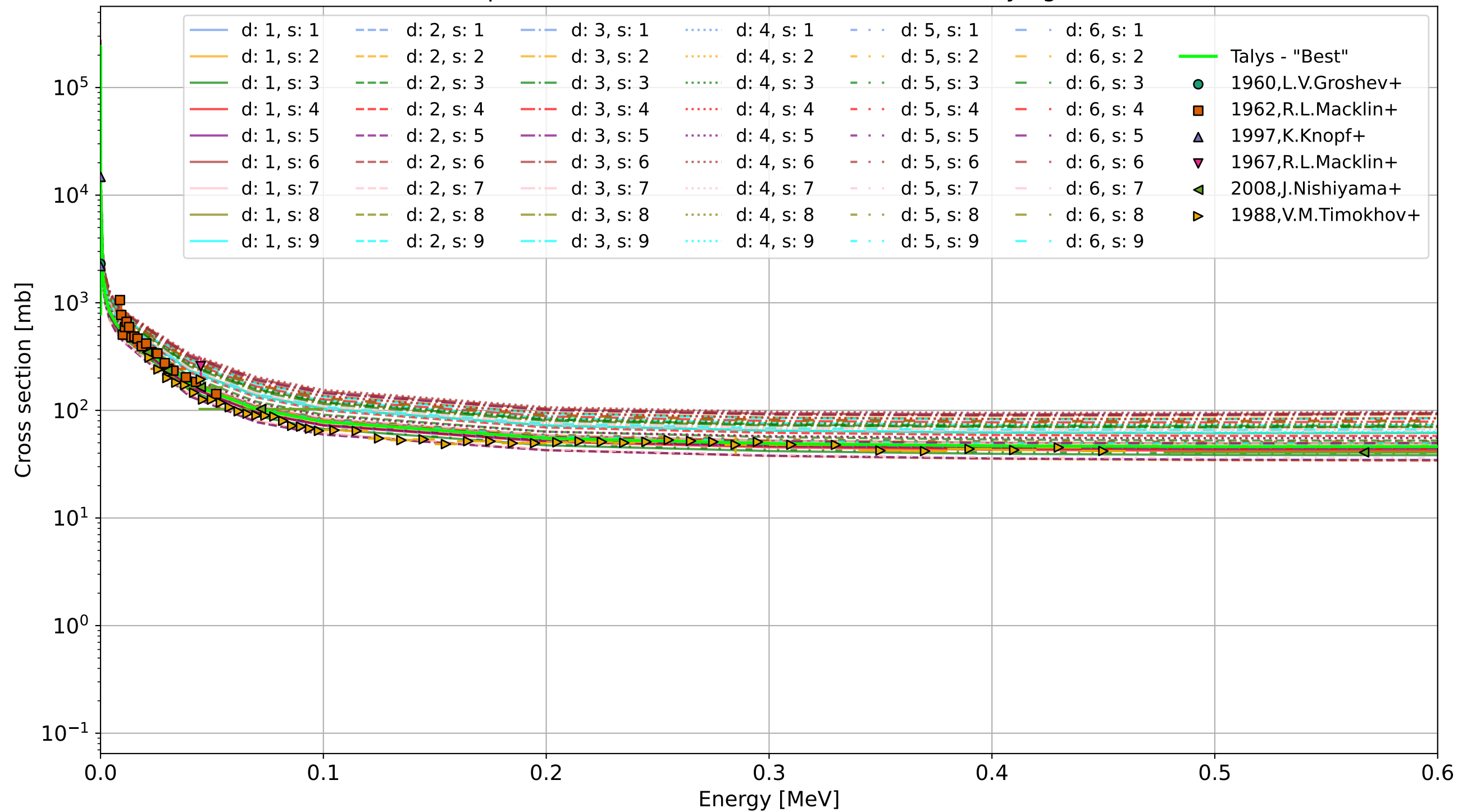
^{119}\text{Sn}(n,\gamma)^{120}\text{Sn} Cross Sections from TALYS with Varying Models
