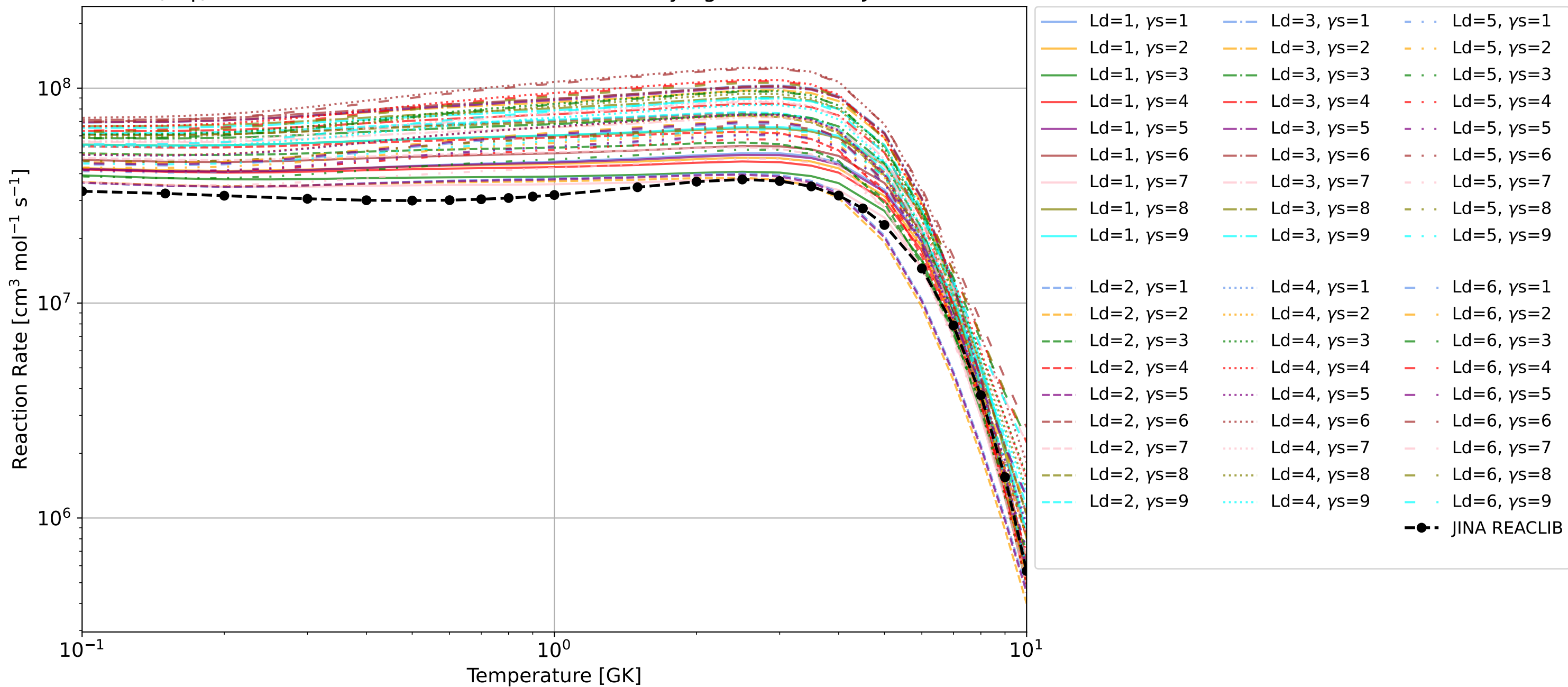
^{119}\text{Sn}(n,\gamma)^{120}\text{Sn} reaction rates from TALYS with varying models and JINA REACLIB
