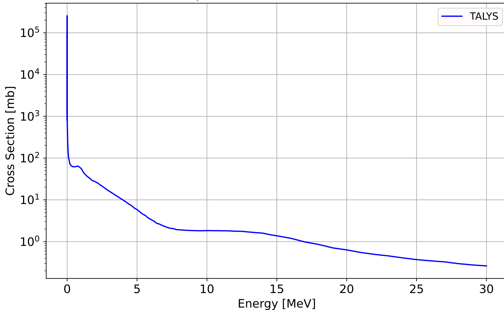
^{121}\text{Sn}(n,\gamma)^{122}\text{Sn} cross section from TALYS
