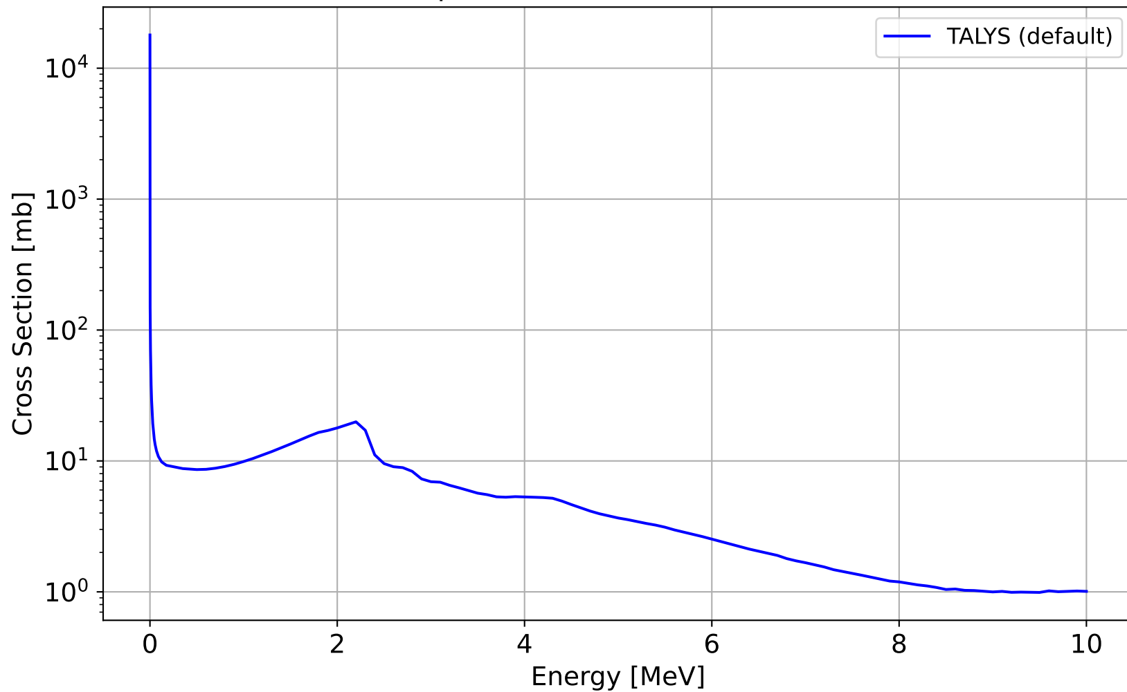
^{90}\text{Zr}(n,\gamma)^{91}\text{Zr} cross section from TALYS
