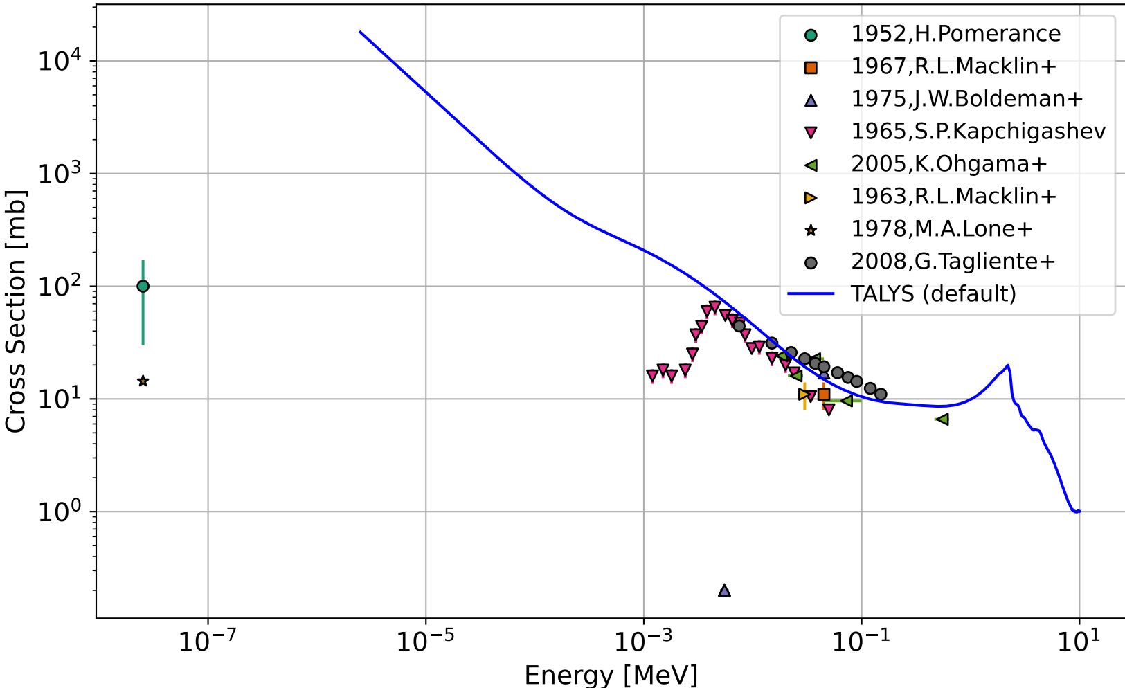
^{90}\text{Zr}(n,\gamma)^{91}\text{Zr} cross section comparison
