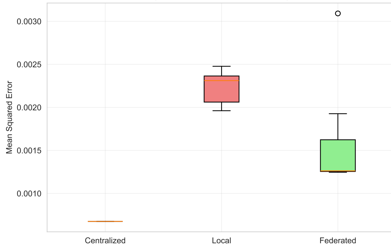
MSE: NerveDysesthesia (Predicted vs True Probabilities)
