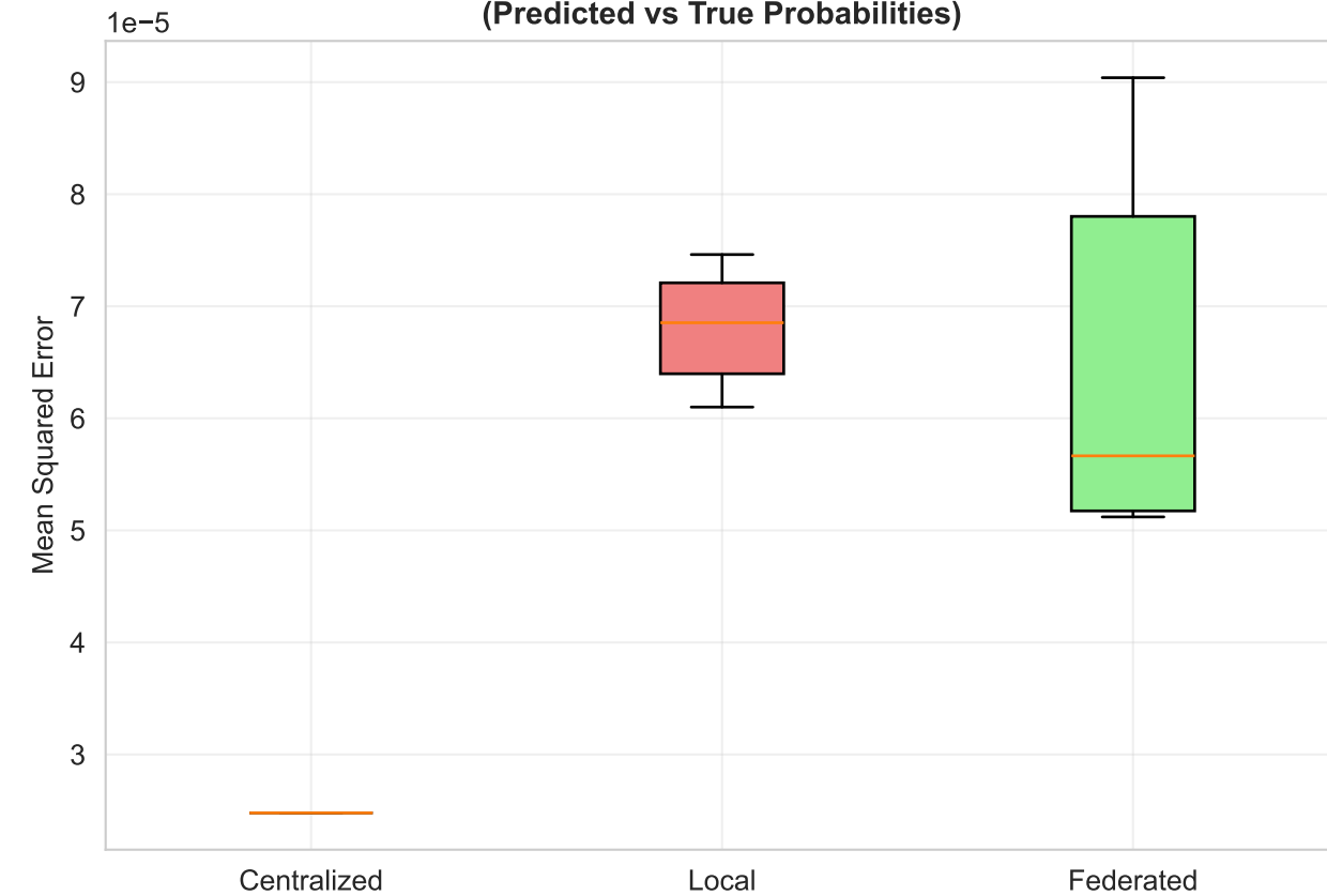
MSE: Bleeding (Predicted vs True Probabilities)
