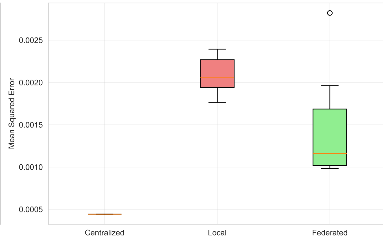
MSE: Bleeding (Predicted vs True Probabilities)
