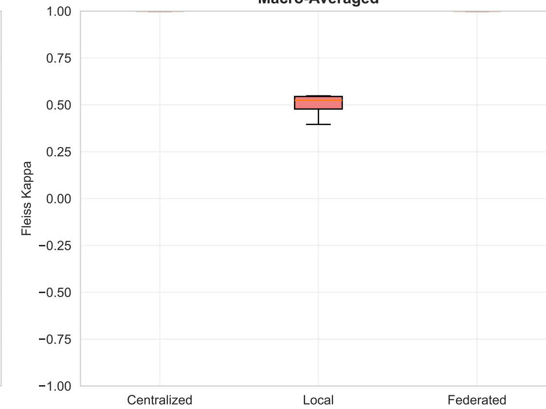
Fleiss Kappa (Global Thresholds) Macro-Averaged
