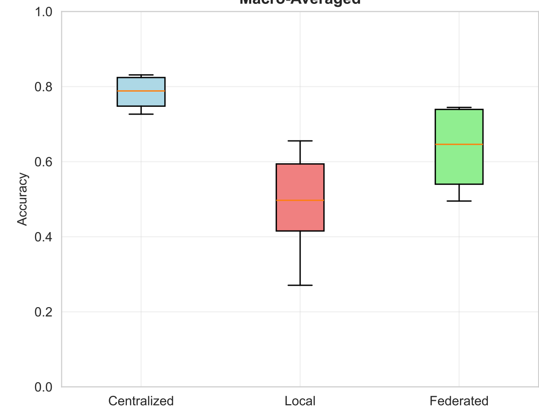
Accuracy (Per-Client Categories) Macro-Averaged
