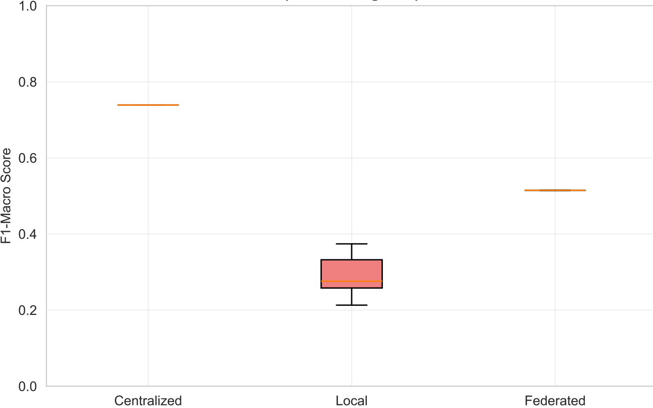
F1-Macro: Bleeding (Global Categories)
