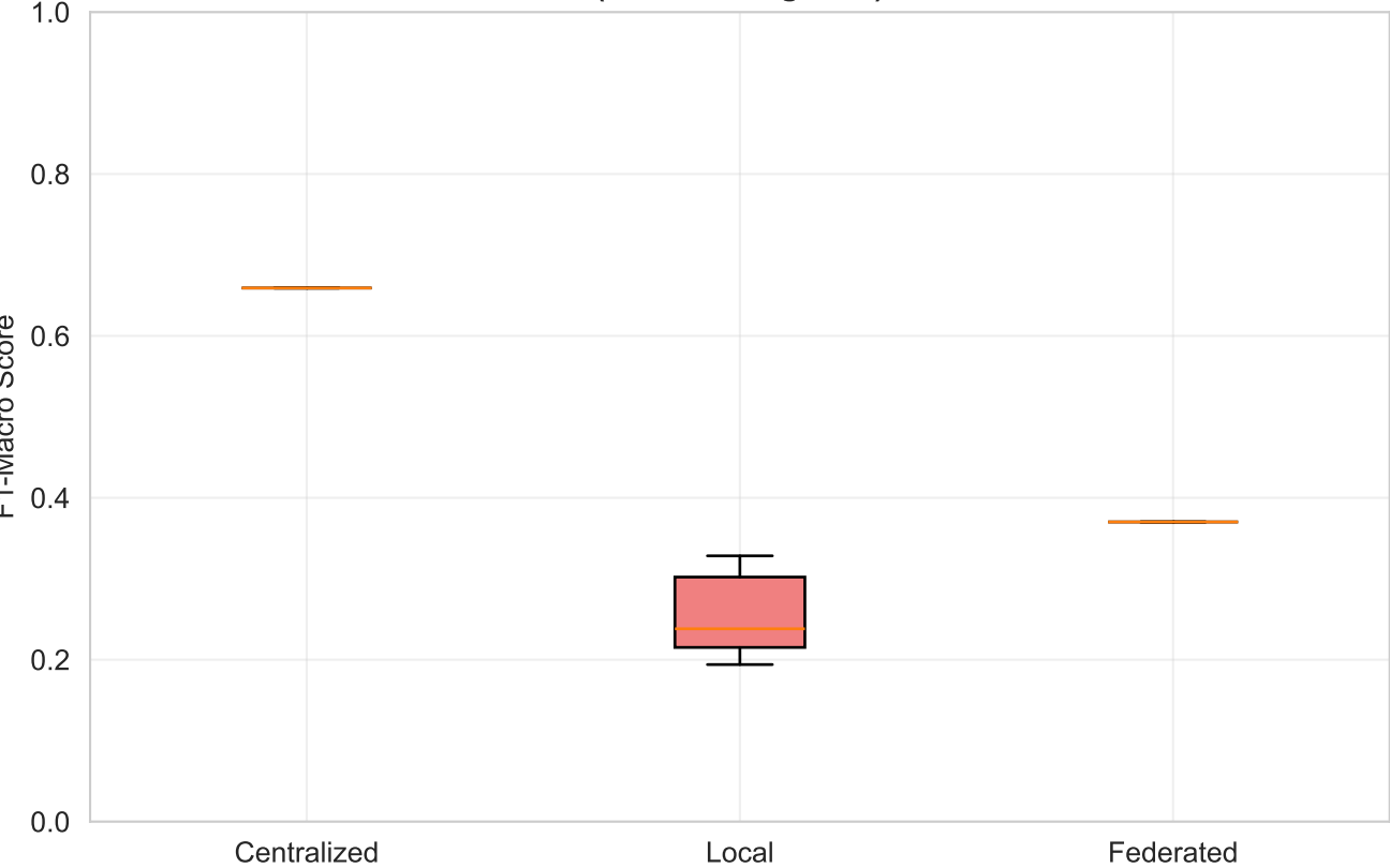
F1-Macro: NerveDysesthesia (Global Categories)
