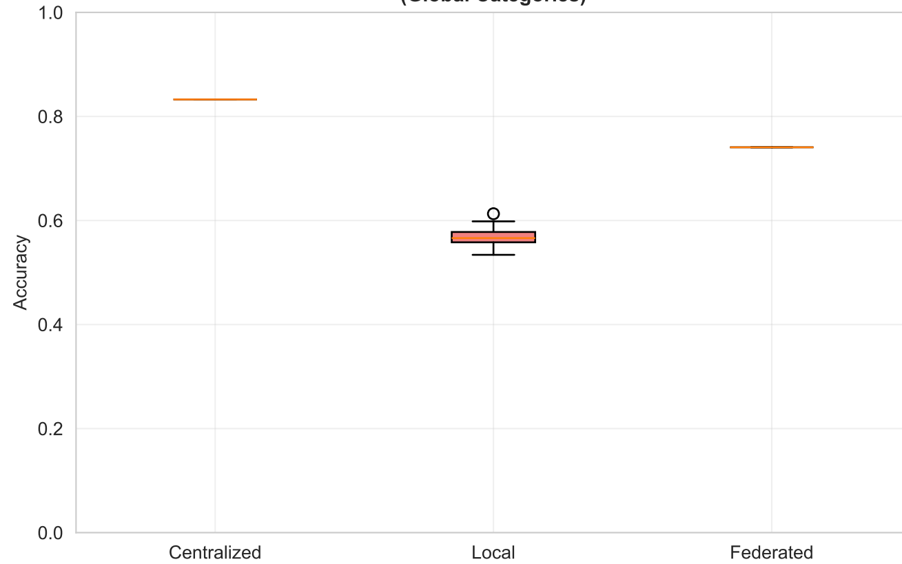
Accuracy: NerveDysesthesia (Global Categories)
