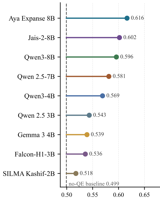
NDCG@10
