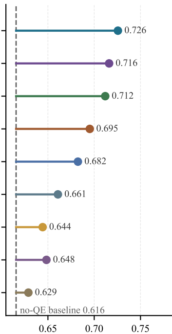
Recall@10
