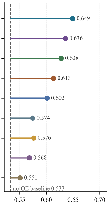
MRR
