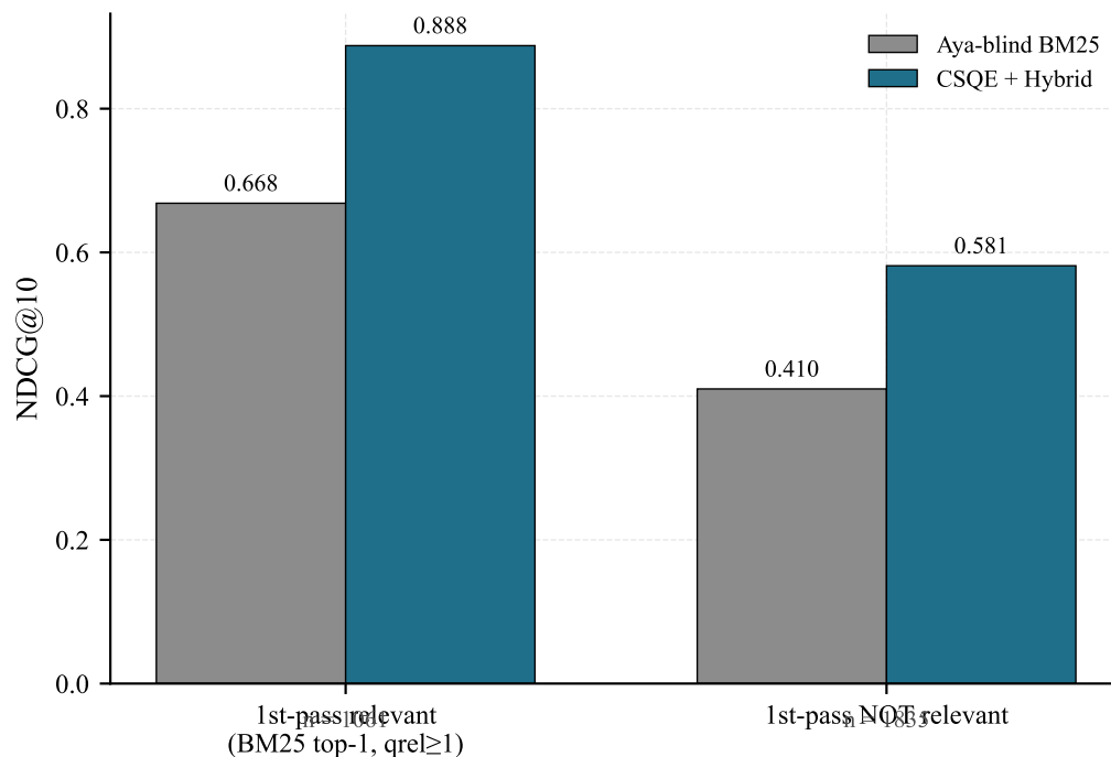
Figure 3.13: CSQE+Hybrid versus Aya-blind baseline conditioned on whether the BM25 first-pass top-1 document is relevant ( \text{qrel} \geq 1 ). When the first-pass document is relevant ( n = 1,061 ) CSQE+Hybrid reaches 0.888 nDCG@10; when it is not ( n = 1,835 ) it reaches 0.581.
