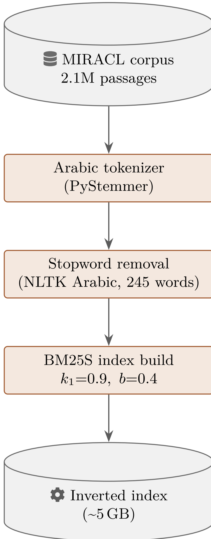
Figure 2.2: BM25S indexing pipeline applied to the MIRACL Arabic corpus. Passages are tokenised with PyStemmer, stopwords-removed using 245 Arabic stopwords, then indexed under BM25S with k_1=0.9 and b=0.4 .
