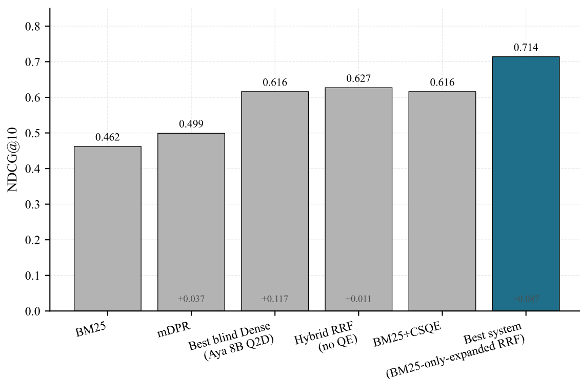
Figure 3.11: Progression of nDCG@10 from the BM25 baseline (0.462) through intermediate query-enhancement steps to the best system, BM25-only-expanded with RRF fusion, at 0.714. The annotation on each bar reports the gain over the best previous configuration.
