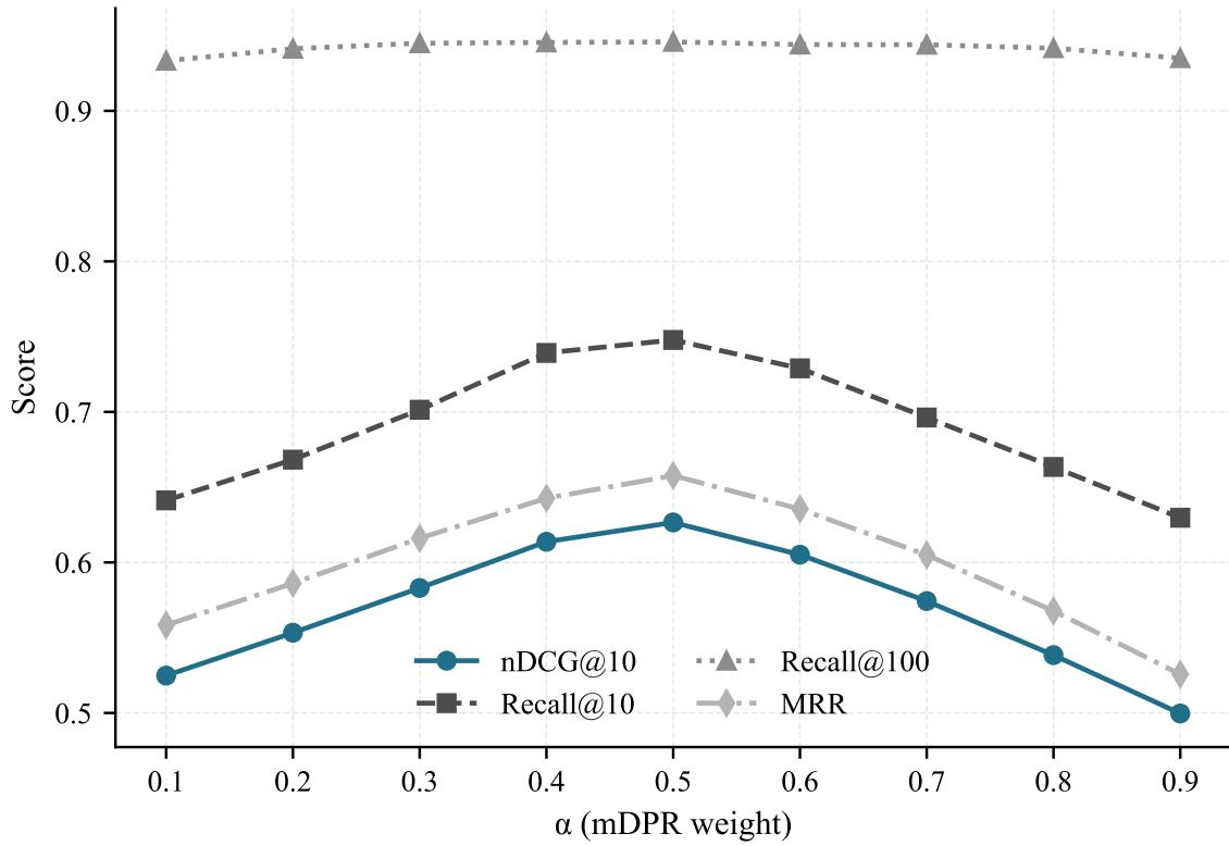
Figure 3.10: Convex-combination \alpha sweep for the no-QE hybrid baseline, showing nDCG@10, Recall@{10,100} and MRR. nDCG@10 peaks near \alpha = 0.5 ; Recall@100 is largely insensitive to \alpha .
