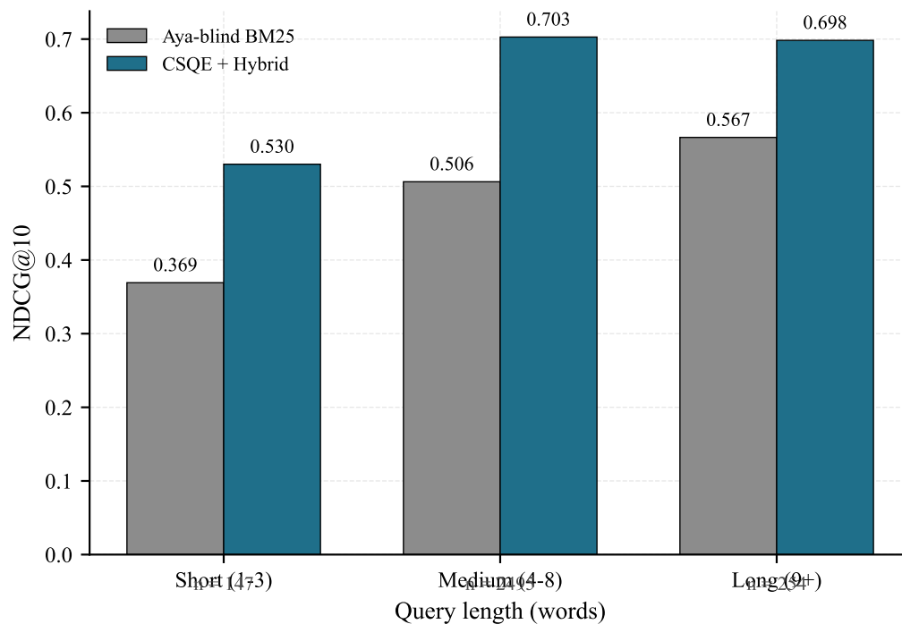
Figure 3.14: Per-bucket comparison of Aya-blind BM25 and CSQE+Hybrid using the 1–3 / 4–8 / 9+ word buckets. CSQE+Hybrid improves every bucket; short queries gain the most proportionally (+43.6%) and medium queries the most absolutely (+0.197).
