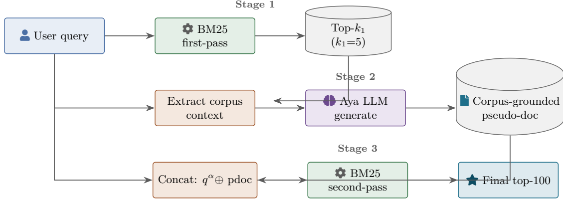
Figure 2.6: Corpus-Steered Query Expansion (CSQE) pipeline. Stage 1: BM25 retrieves a first-pass top- k_1 context. Stage 2: corpus context plus the original query are fed to the Aya LLM, which generates a corpus-grounded pseudo-document. Stage 3: the query (repeated \alpha times) is concatenated with the pseudo-document and fed to a BM25 second pass.
