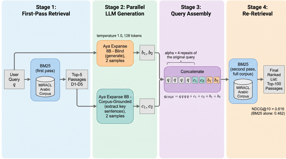
Figure 3.6: CSQE pipeline. Stage 1: BM25 retrieves the top- k_1 = 5 passages D_1 \dots D_5 for query q . Stage 2: Aya Expanses 8B generates two independent, parallel branches at temperature 1.0 (128 tokens each) — a blind branch that sees q only and generates b_1, b_2 from parametric knowledge, and a corpus-grounded branch that sees D_1 \dots D_5 and extracts c_1, c_2 . Stage 3: plain string concatenation (no scoring or re-ranking) assembles q_{CSQE} = q q q q + c_1 + c_2 + b_1 + b_2 , with q repeated \alpha = 4 times to counter BM25 term dilution. Stage 4: q_{CSQE} drives a fresh BM25 pass over the full corpus, yielding NDCG@10 = 0.616 (BM25 with raw q : 0.462).
