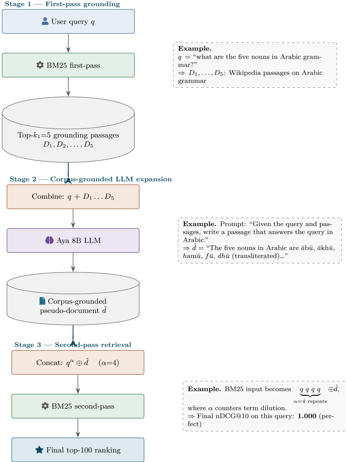
Figure 3.6: Corpus-Steered Query Expansion (CSQE) pipeline. Stage 1: BM25 retrieves a first-pass top- k_1 context. Stage 2: corpus context plus the original query are fed to the Aya LLM, which generates a corpus-grounded pseudo-document. Stage 3: the query (repeated \alpha times) is concatenated with the pseudo-document and fed to a BM25 second pass.
