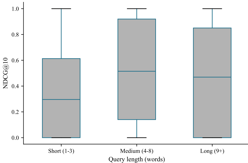
Figure 4.3: Distribution of mDPR NDCG@10 within each query-length bucket. Short queries clearly underperform, motivating query enhancement as a remedy for information poverty in short queries.
