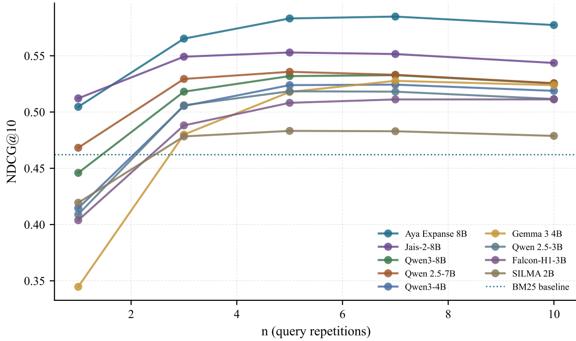
Figure 4.8: n\text{DCG}@10 on the BM25 retriever as a function of query-repetition count n for each LLM-generated pseudo-document. Six of nine models start below the BM25 baseline at n=1 ; all nine recover or exceed it at their optimum n . Colours match Figure 4.5.
