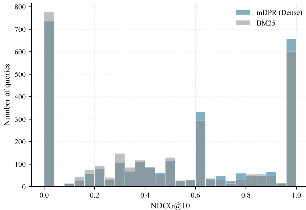
Figure 4.1: Per-query NDCG@10 distribution for the two baseline retrievers on the MIRACL Arabic dev set. Both exhibit a bimodal distribution: a large mass near zero (poorly served queries) and another mass near one (perfectly served), with relatively few in between.
