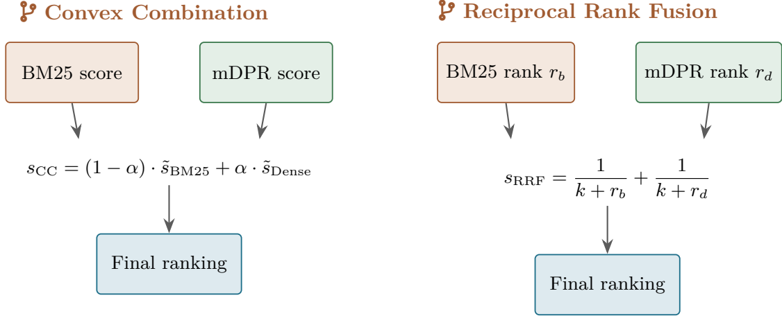
Figure 3.5: Two retriever-fusion methods evaluated in this thesis. Convex Combination (left) computes a weighted sum of normalised retrieval scores; Reciprocal Rank Fusion (right) sums the reciprocal of each retriever’s rank for every document.
