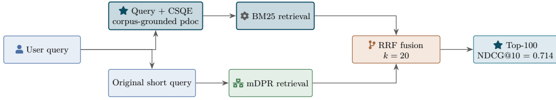
Figure 3.7: Architecture of the thesis’s best-performing system. CSQE-expanded queries are fed to BM25 while the original short queries are fed to mDPR; the two ranked lists are fused with Reciprocal Rank Fusion ( k = 20 ), yielding the headline nDCG@10 of 0.714.
