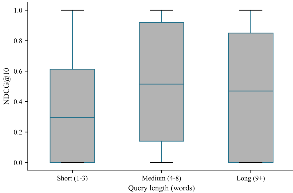
Figure 4.3: Distribution of mDPR \text{NDCG@10} within each query-length bucket. Short queries clearly underperform, motivating query enhancement as a remedy for information poverty in short queries.
