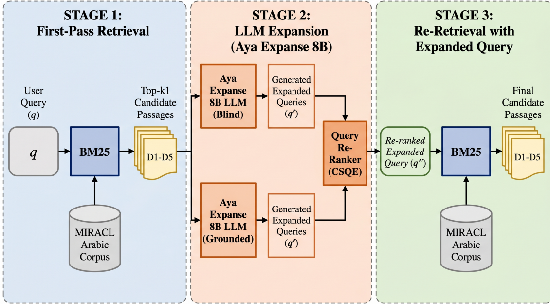
Figure 3.6: CSQE pipeline. Stage 1: BM25 retrieves the top- k_1 = 5 first-pass passages. Stage 2: Aya Expanse 8B is invoked four times ( \alpha = 4 , temp = 1.0): two corpus-grounded calls ( c_1, c_2 ) extract key sentences from the retrieved passages; two blind calls ( b_1, b_2 ) generate from parametric knowledge. Stage 3: the original query (repeated \alpha times) is concatenated with all four pseudo-documents and fed to a BM25 second pass, yielding \text{nDCG@10} = 0.616 .
