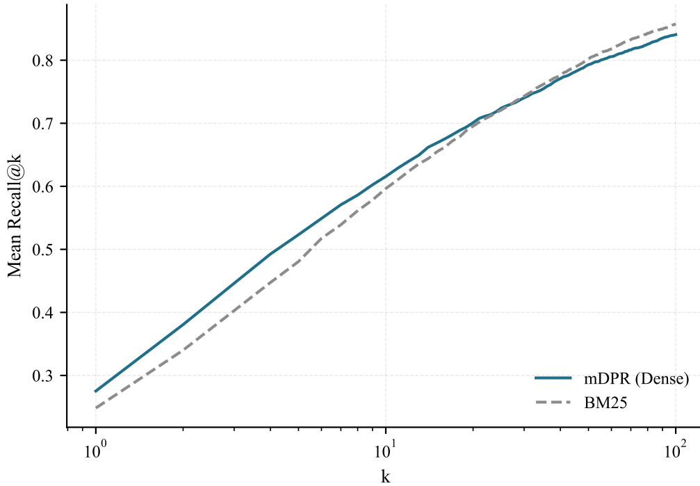
Figure 4.4: Mean \text{Recall}@k for mDPR and BM25 on the MIRACL Arabic dev set, k on a log axis.
