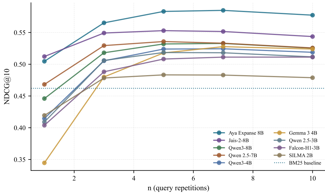
Figure 4.8: NDCG@10 on the BM25 retriever as a function of query-repetition count n for each LLM-generated pseudo-document. Six of nine models start below the BM25 baseline at n=1 ; all nine recover or exceed it at their optimum n . Colours match Figure 4.5.
