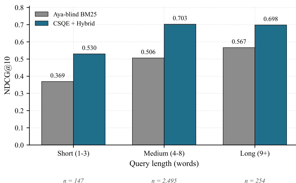
Figure 4.14: Per-bucket comparison of Aya-blind BM25 and CSQE+Hybrid using the 1–3 / 4–8 / 9+ word buckets. CSQE+Hybrid improves every bucket; short queries gain the most proportionally (+43.6%) and medium queries the most absolutely (+0.197).
