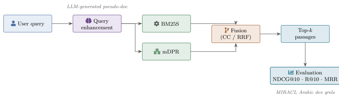
Figure 3.1: Overview of the experimental pipeline. A user query passes through the QE layer; BM25S and mDPR retrieve independently; their ranked lists are fused (CC or RRF) and the top- k passages are scored against the MIRACL Arabic dev qrels. The QE module is the variable component across experiments; the retrieval and evaluation components remain fixed.
