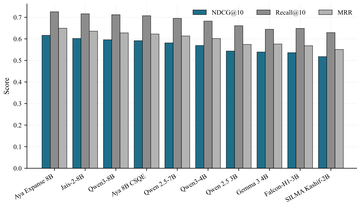
Figure 4.6: Grouped per-model bars for NDCG@10, Recall@10 and MRR on the Query2Doc dense pipeline; same model ordering as Figure 4.5.
