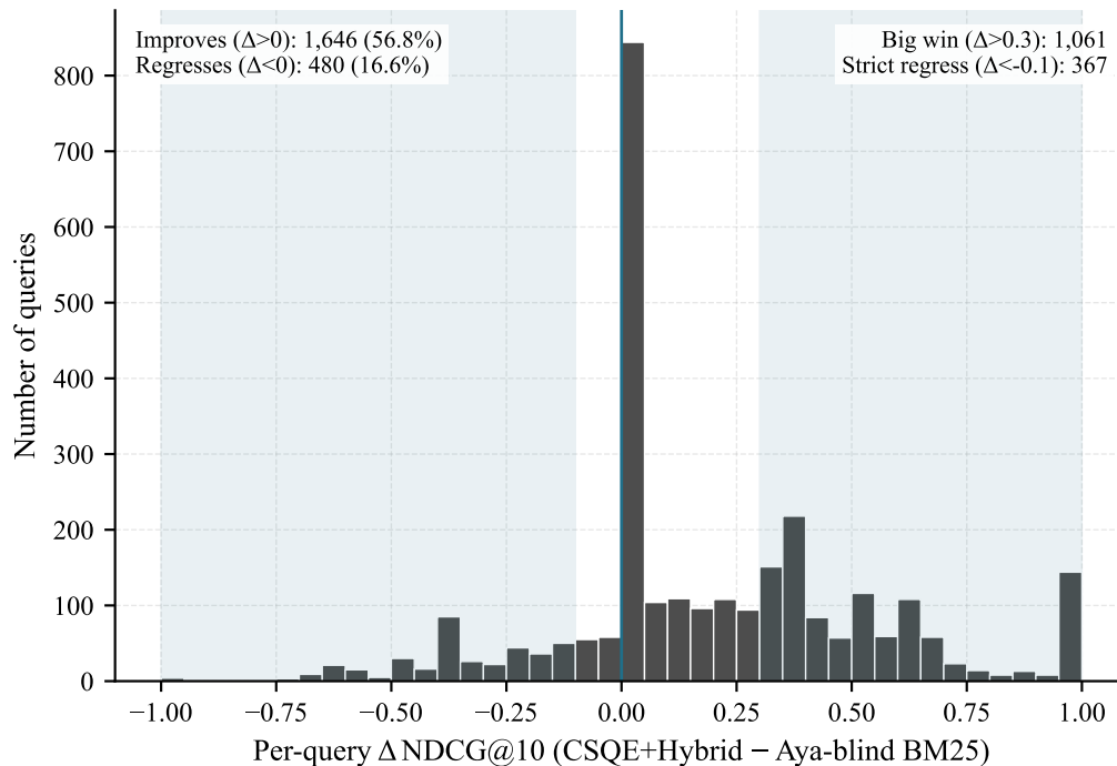
Figure 4.12: Distribution of the per-query difference \Delta = \text{NDCG@10}(\text{CSQE+Hybrid}) - \text{NDCG@10}(\text{Aya-blind BM25}) across all 2,896 MIRACL Arabic dev queries. Shaded bands mark the Big-Win region ( \Delta > 0.3 ) and the strict Regression region ( \Delta < -0.1 ).
