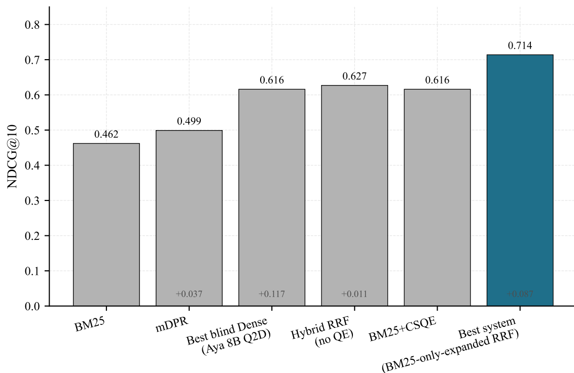
Figure 4.11: Progression of NDCG@10 from the BM25 baseline (0.462) through intermediate query-enhancement steps to the best system, BM25-only-expanded with RRF fusion, at 0.714. Annotations on each bar report the gain over the best previous configuration.
