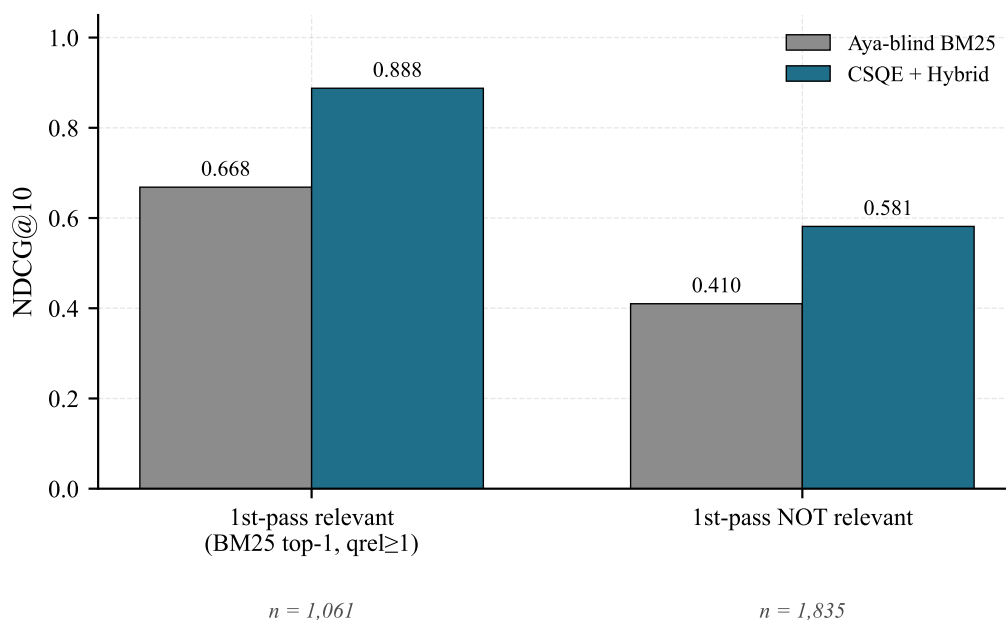
Figure 4.13: CSQE+Hybrid versus Aya-blind BM25 baseline conditioned on whether the BM25 first-pass top-1 document is relevant ( qrel \geq 1 ). The asymmetry between the relevant ( n = 1,061 ) and not-relevant ( n = 1,835 ) groups demonstrates first-pass quality as the largest behavioural modulator of CSQE.
