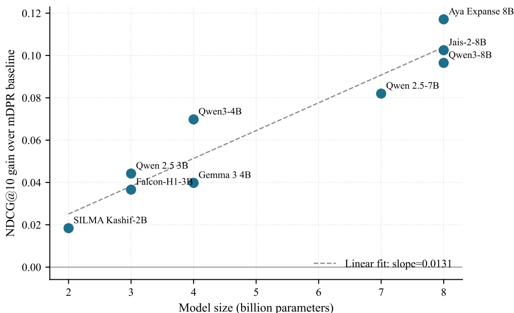
Figure 4.7: Relationship between model parameter count (billions) and gain over the mDPR baseline. A weak positive trend is visible across the full set, and the Qwen-family subset corroborates the size–quality correlation within a single architecture. ALLaM-7B is excluded as an outlier due to tokeniser artefacts.
