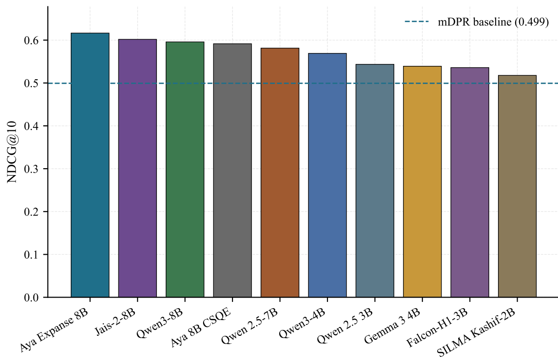
Figure 4.5: Dense retrieval NDCG@10 for all evaluated LLMs on the Query2Doc pipeline, sorted descending. The dashed reference line marks the mDPR no-QE baseline (0.499); each model uses its consistent thesis colour, matching Figure 4.8.
