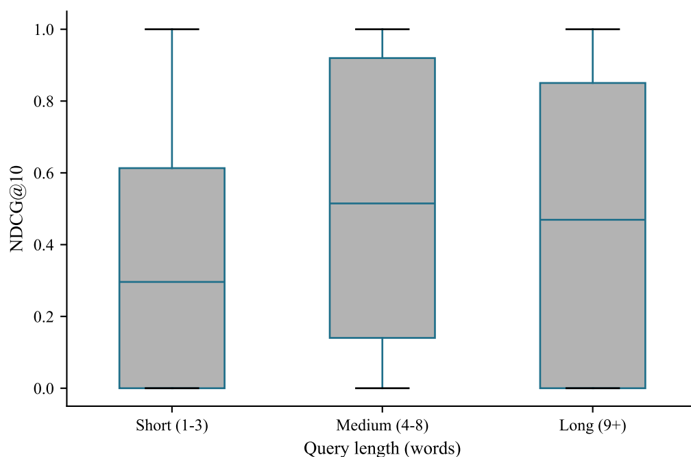
Figure 4.3: Distribution of mDPR NDCG@10 within each query-length bucket. Short queries clearly underperform, motivating QE as a remedy for information poverty in short queries.
