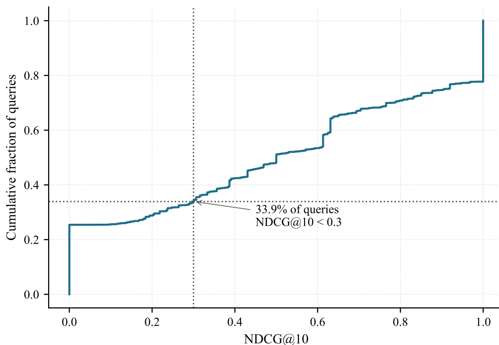
Figure 4.2: Cumulative distribution of per-query NDCG@10 on the mDPR baseline. The annotated threshold at 0.3 separates the failed queries from the remainder.
