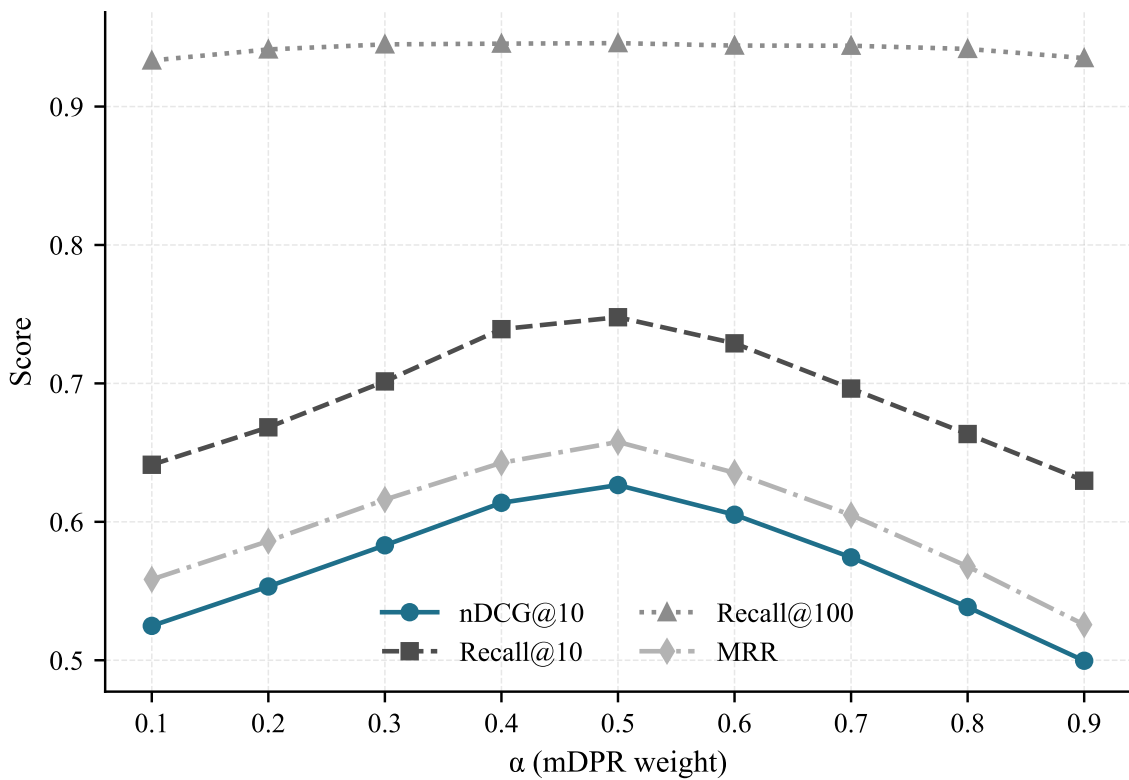
Figure 4.10: Convex-combination \alpha sweep for the no-QE hybrid baseline, showing NDCG@10, Recall@{10,100} and MRR. NDCG@10 peaks near \alpha = 0.5 ; Recall@100 is largely insensitive to \alpha .
