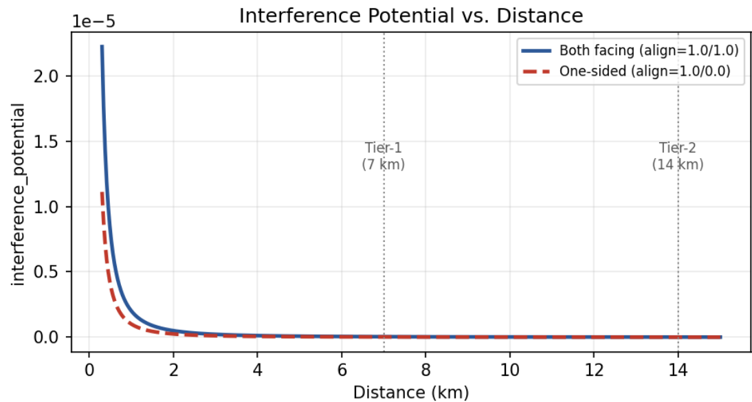
Fig. 3.3: Interference potential vs. distance for a fully-facing pair (both alignments = 1.0) and a one-sided pair (only one antenna facing). Tier-1 (7 km) and Tier-2 (14 km) boundaries are marked for reference. ig:pi-interference-distance
