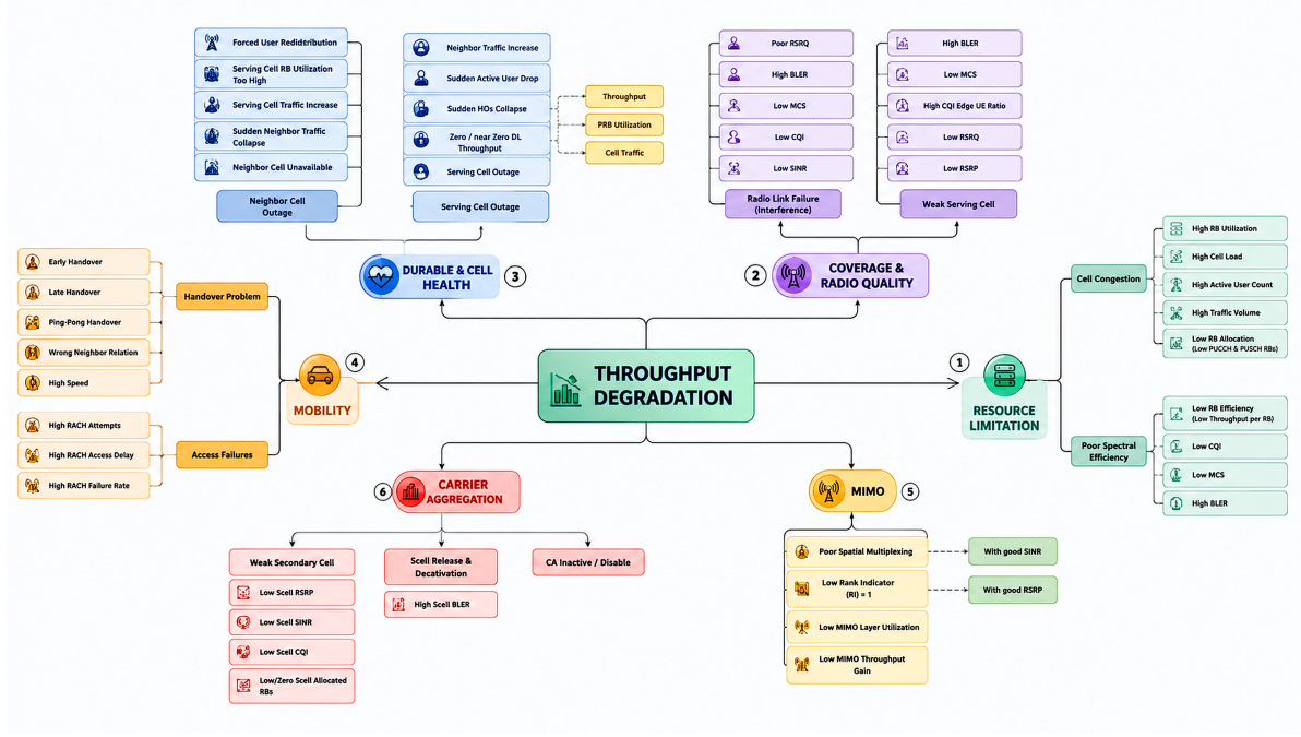
Fig. 2.2: Engineering RCA cause taxonomy for LTE throughput degradation and the supporting KPI/evidence branches.
