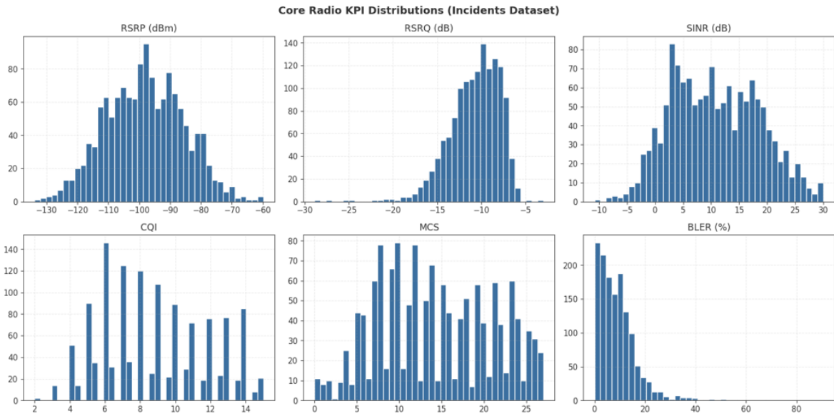
Fig. 2.1: Core radio KPI distributions across the incident dataset: RSRP, RSRQ, SINR, CQI, MCS, and BLER.
