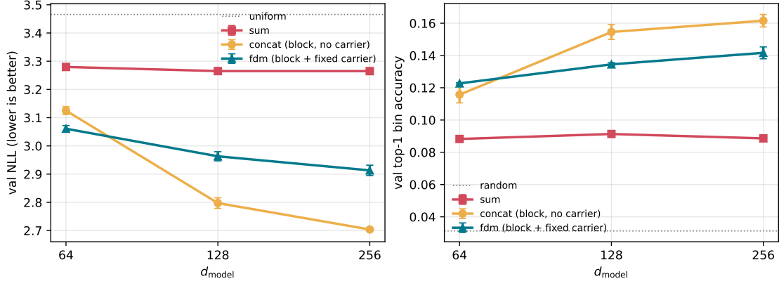
Figure 2: Scaling with d_{\text{model}} at C=4 . SUM is essentially flat: extra width buys nothing because the bottleneck is structural, not representational. CONCAT and FDM both improve, but CONCAT improves more—the fixed carrier becomes a constraint once the per-channel block is wide enough to learn its own temporal structure.
