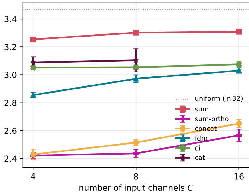
val NLL (lower is better)
