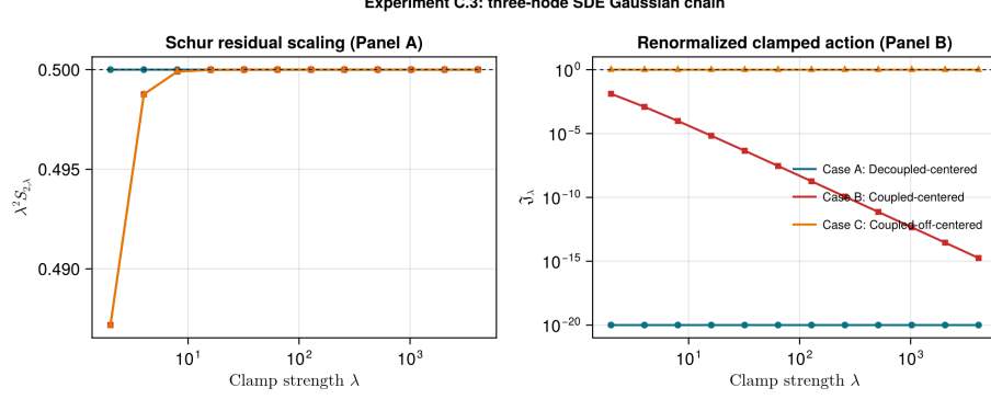
Figure F.3: The panels show \lambda^2 S_{2,\lambda} \rightarrow 0.5 and the three finite-part regimes: exact zero, O(\lambda^{-4}) decay, and convergence to 1.
