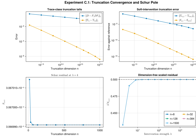
Figure F.1: Trace-norm and residual errors decay in n ; the extrapolated m_2^{\text{Schur},(1000)} differs from \varepsilon_0/2 by 6.87 \times 10^{-14} .
