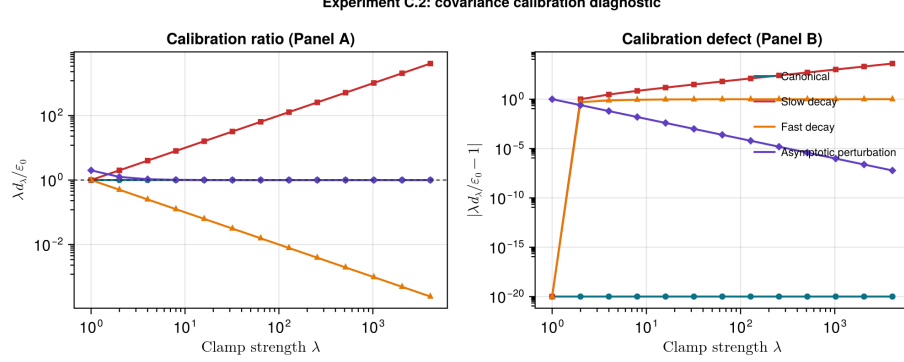
Figure F.2: The perturbed family has the correct limiting ratio but fails the exact finite- \lambda covariance condition. Exact zero defects are displayed at 10^{-20} .
