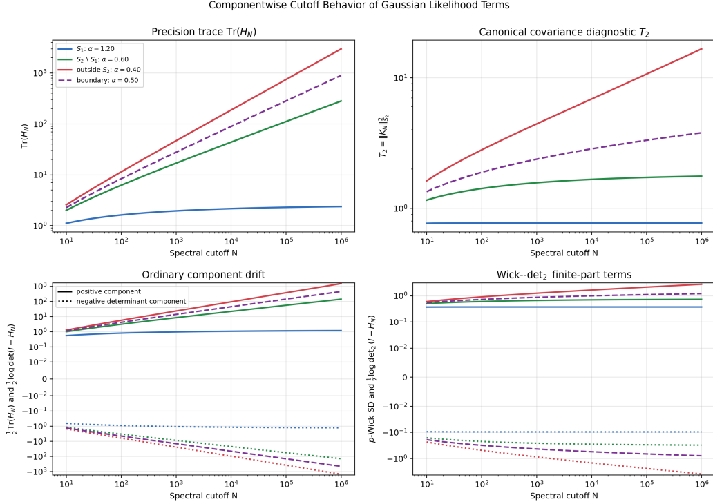
Figure 1: The operator-ideal boundary appears only under refinement. Power-law precision spectra traverse S_1 , S_2 \setminus S_1 , the critical boundary, and the non- S_2 regime. The top-right panel reports the canonical covariance diagnostic \|K_N\|_{S_2}^2 ; the precision bridge in Section B gives the same phase boundary for H_N . Ordinary components drift separately, while the Wick- \det_2 finite part and its stochastic fluctuation remain controlled on the bounded side.
