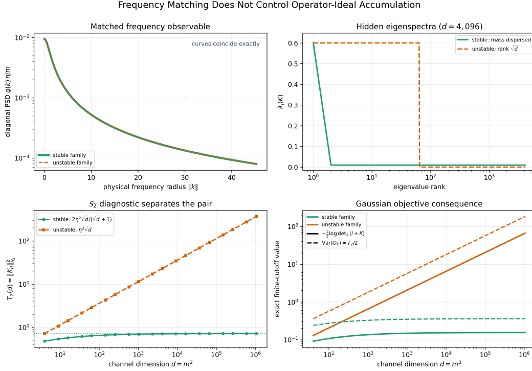
Figure 1: Frequency matching does not control operator-ideal accumulation. The two families have identical radial Fourier diagonals, trace, and operator norm, but different hidden eigenvalue multiplicities. At d = 1,048,576 , the stable family has T_2 = 0.7193 , while the unstable family reaches 368.64, a 512.5\times separation inherited by the exact Gaussian residue and centered quadratic variance. All curves are closed-form; explicit DFT matrices verify the identities at small d .
