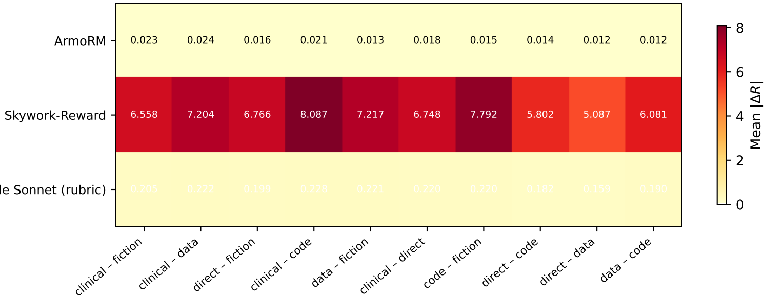
Format-pair sensitivity by judge (mode b)
