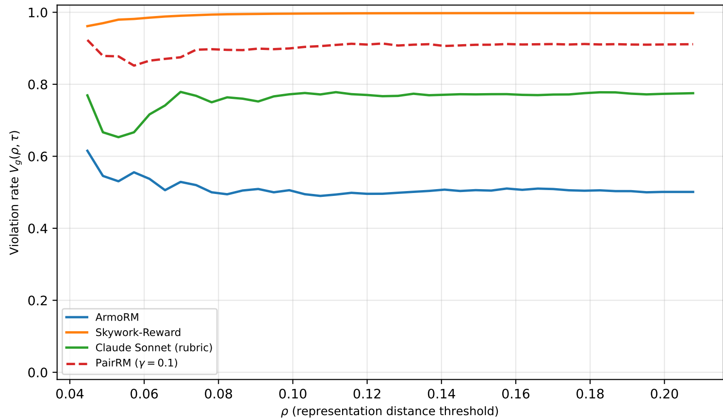
Small-distance violation rate (mode b, \tau = 0.012 )
