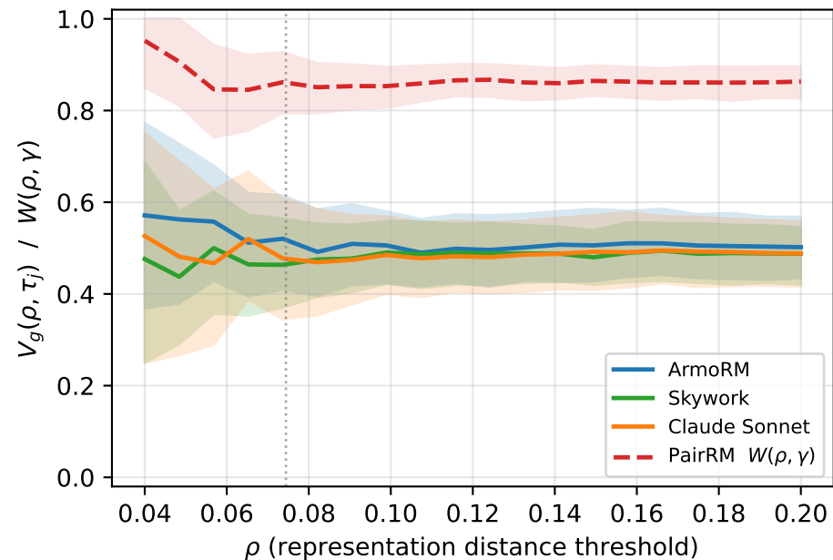
Conditional violation rate
