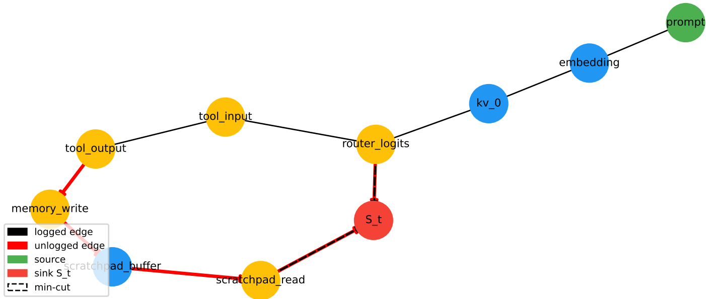
Deployment DAG: react_agent_extracted
