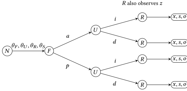
Fig. 1. Extensive-form skeleton of the signaling game. Nature draws private types; F signals first, U responds, and R acts after observing both public messages and the noisy public signal z .
