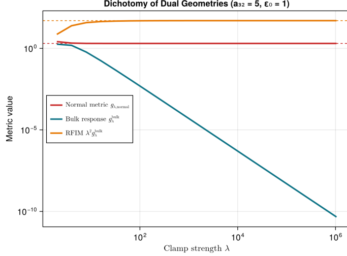
FIGURE 4. Dichotomy of dual geometries for the 3-node serial Gaussian chain under target coordinate conditioning on X_2 ( \varepsilon_0 = 1 , a_{32} = 5 ). The 0th-order normal metric g_{\lambda,\text{normal}} (red) instantly stabilizes at the horizontal plateau 2/\varepsilon_0 = 2 , showing the survival of the boundary geometry. The unrenormalized horizontal lift response g_{\lambda}^{\text{bulk}} (blue) collapses strictly at a slope of -2 as O(\lambda^{-2}) . Rescaling the bulk response by \lambda^2 yields the 1st-order metric (orange), which locks onto the non-zero Cameron–Martin limit \|a_{Ik}\|_{Q_0^{-1}}^2 = 2a_{32}^2 = 50 .
