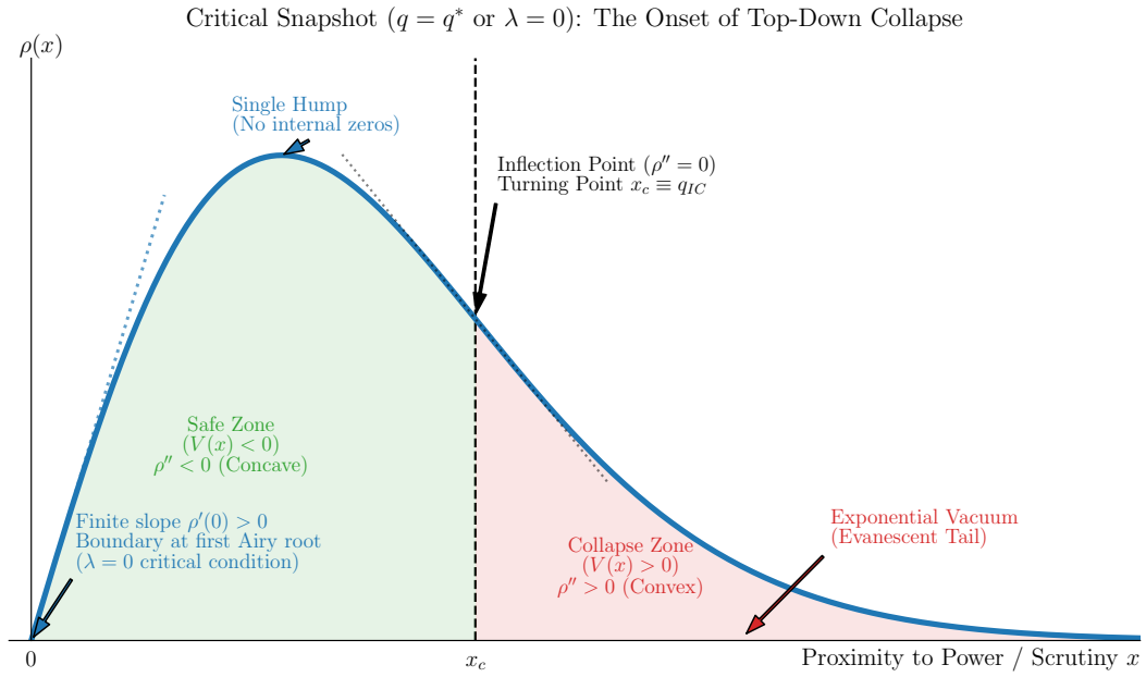
Figure 2: The critical snapshot at q = q^* , equivalently \lambda = 0 . The stationary cross-sectional density forms a single hump anchored in the protected region. At the critical cut x_c , the profile passes through the knife-edge between positive stationary occupancy and spectral nonexistence. The supercritical top-end vacuum is asserted only for \lambda < 0 .
