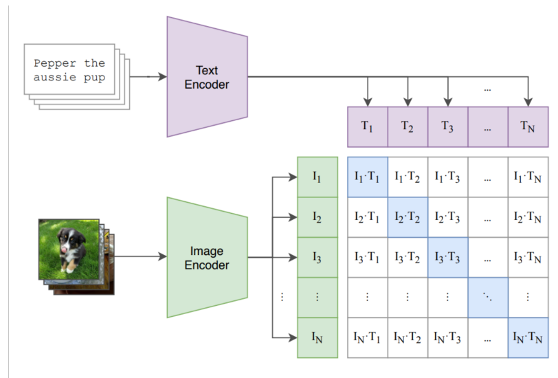
Figure 2.13. Illustration of the contrastive pretraining process, where corresponding batches of images and their textual descriptions are jointly trained to predict correct pairings [95].
