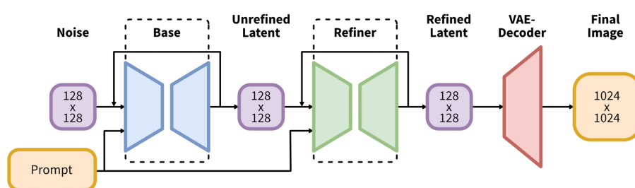
Figure 2.15. Illustration of the two-stage SDXL pipeline. The one-stage model is the same, but without the refiner and its output refined latent. [139]
