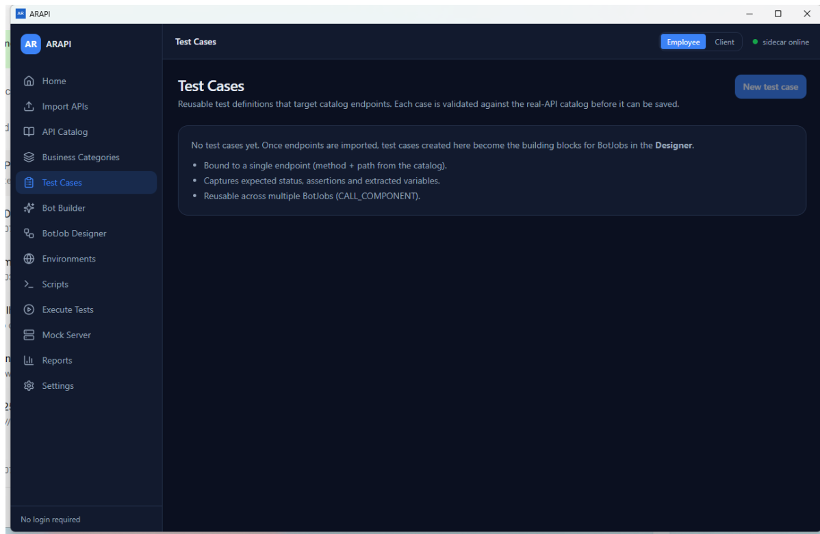
Figure 6. Test Cases
