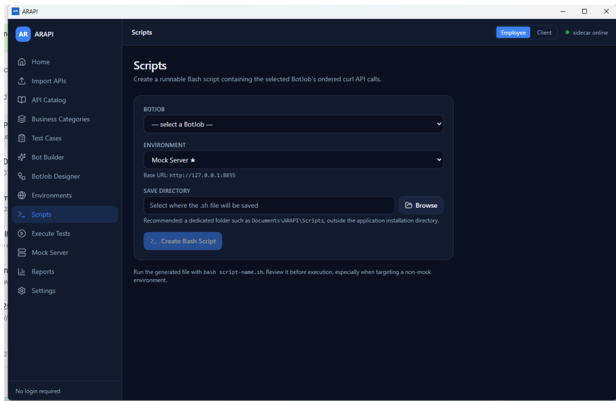
Figure 14. Scripts - initial
