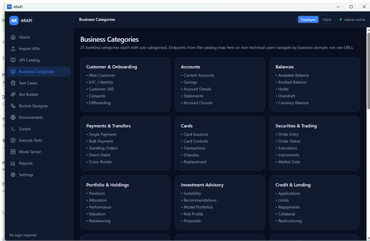
Figure 5. Business Categories
