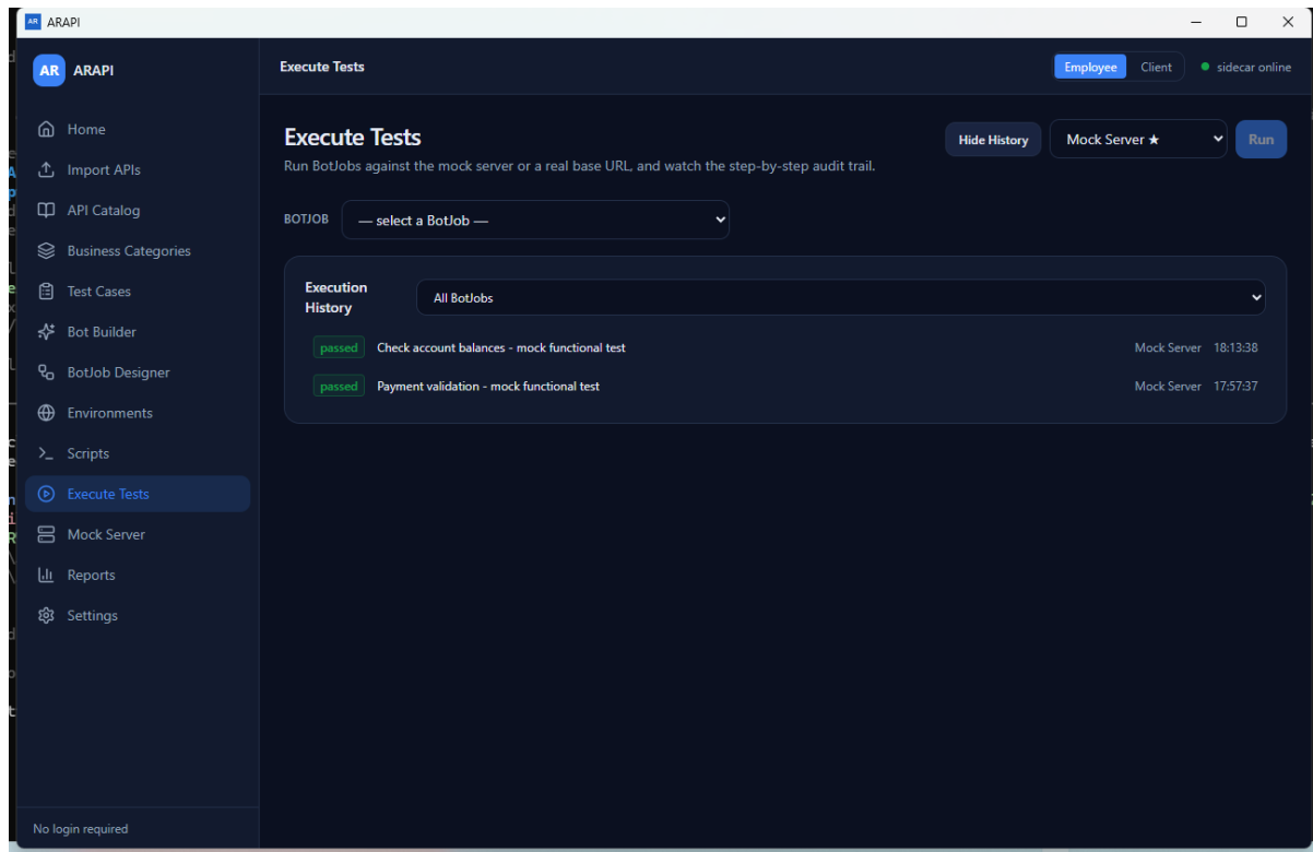
Figure 20. Execution History
