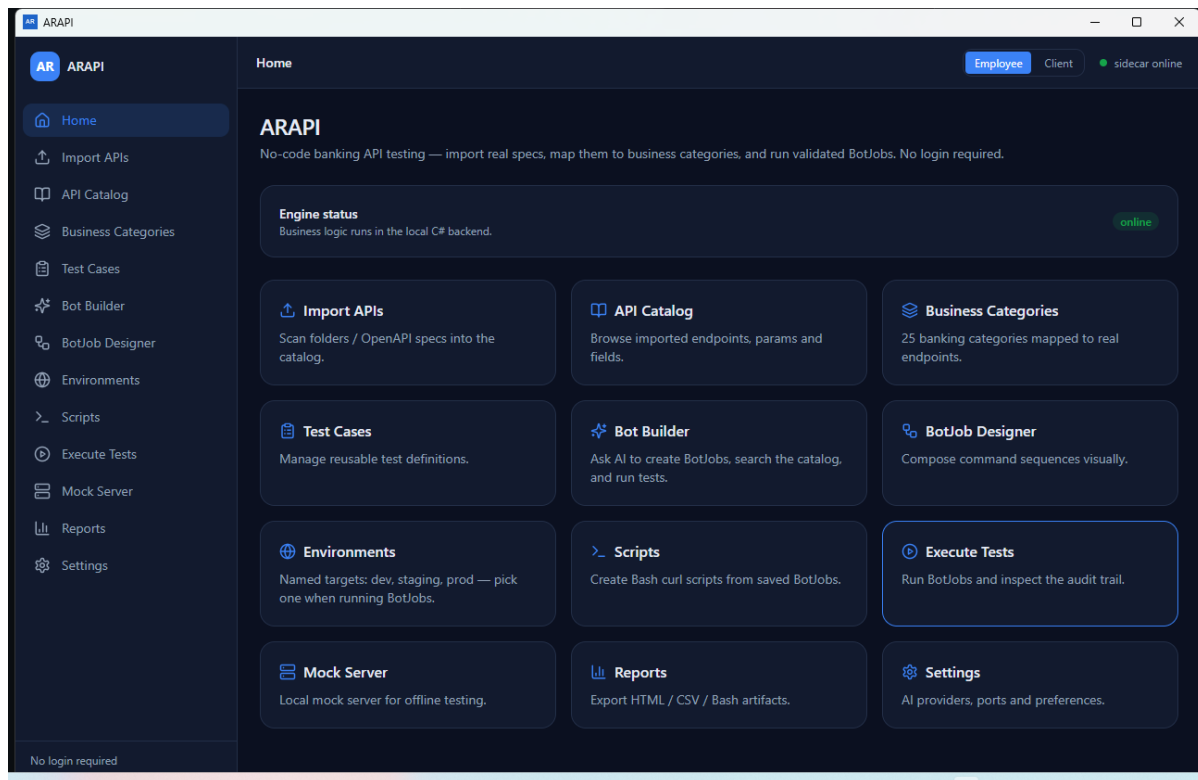
Figure 1. Home overview
