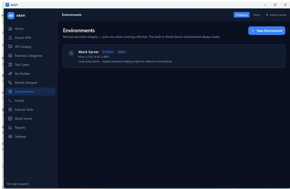
Figure 12. Environments
