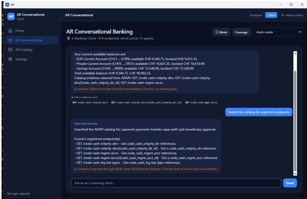
Figure 9. ARAPI catalog-search delegation
