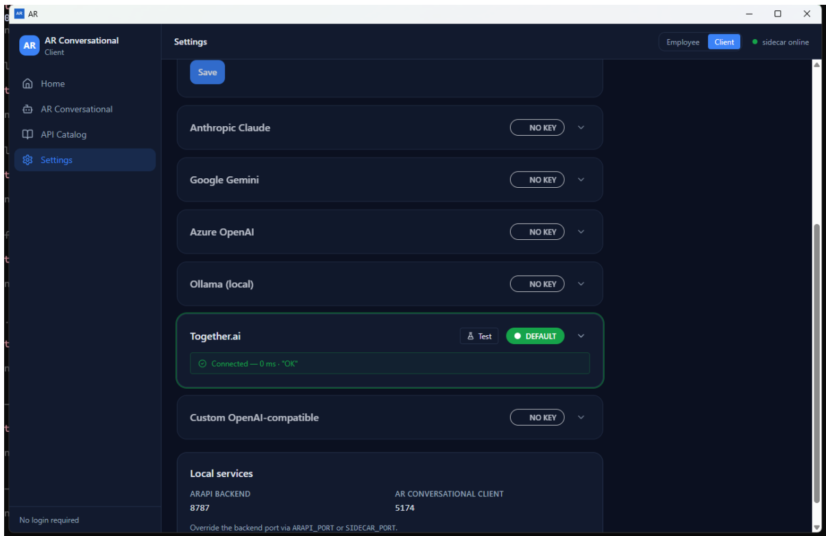
Figure 15. Provider Test result
