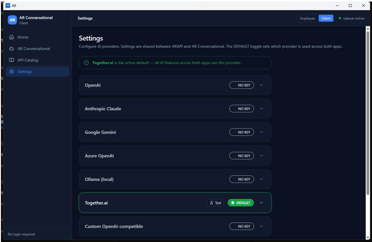
Figure 12. Settings provider list
