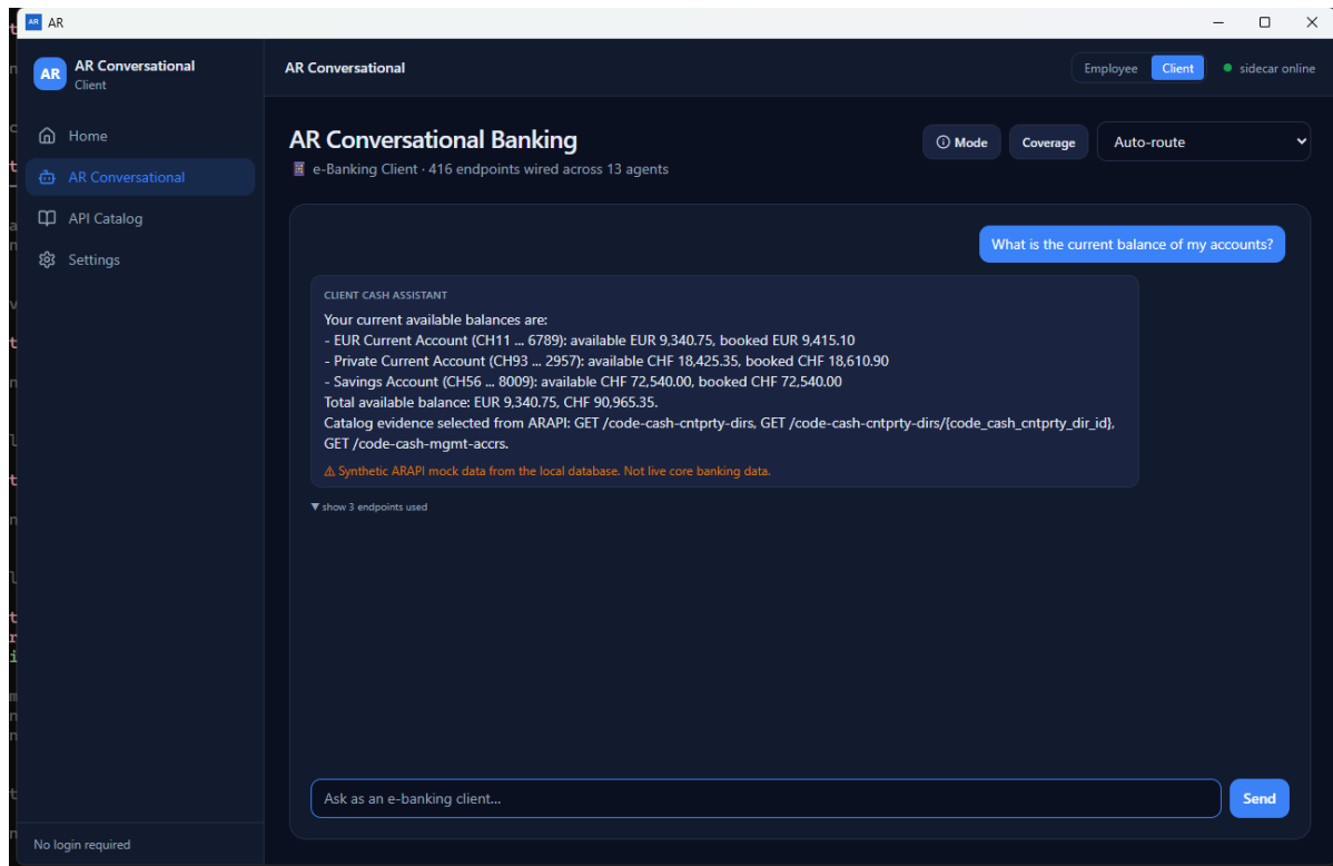
Figure 7. Synthetic client balance answer
