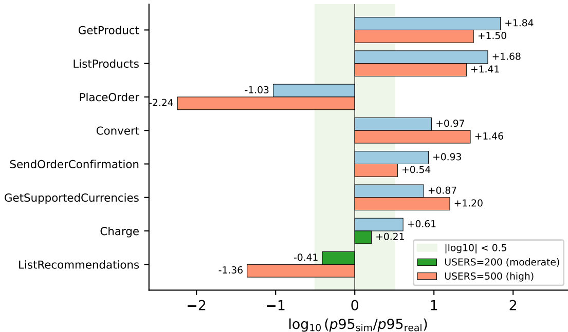
Per-operation latency fidelity, two load levels
