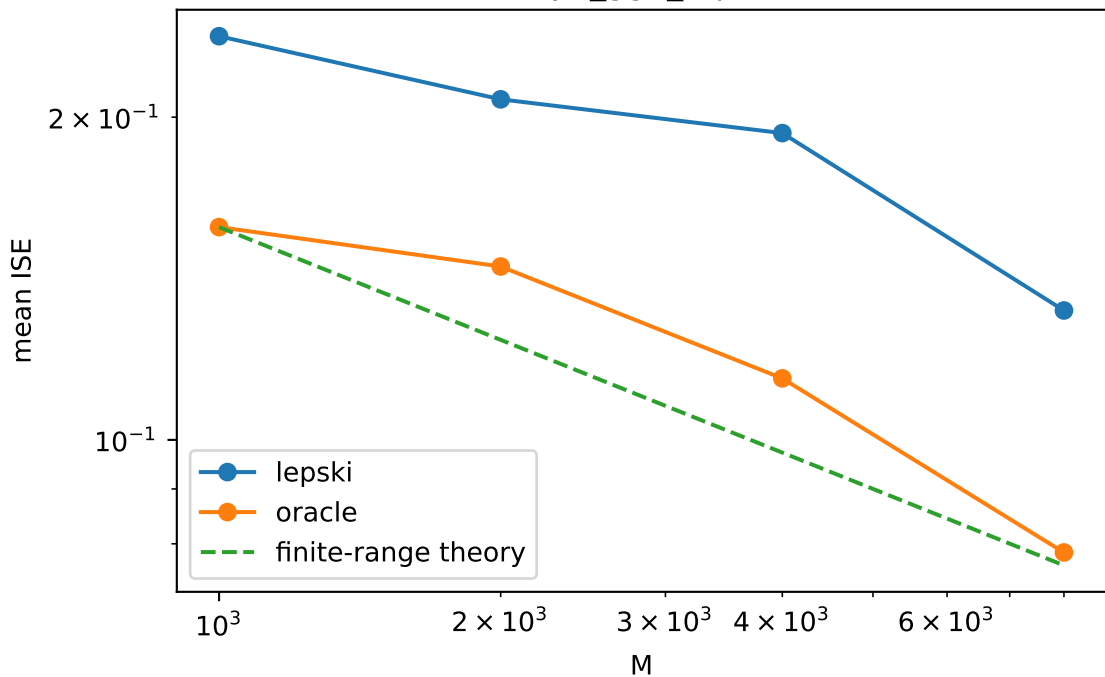
GG 1D (day2_gg1_reproduction)
