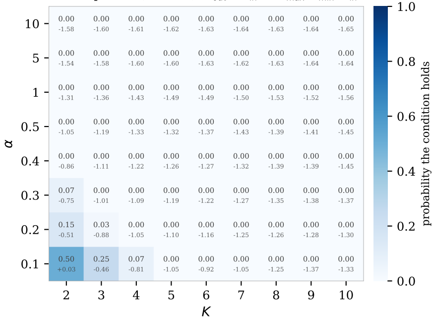
Assumption 5 (balance): \Delta_{\text{out}} - \Delta_{\text{in}} > (w_{\text{max}}/w_{\text{min}}) \Delta_{\text{in}}
