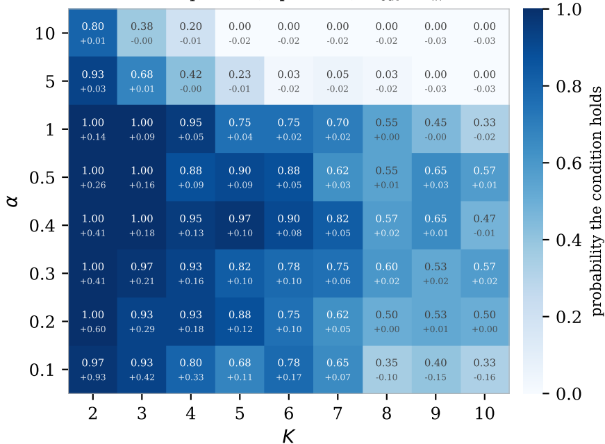
Assumption 3 (separation): \Delta_{\text{out}} > \Delta_{\text{in}}
