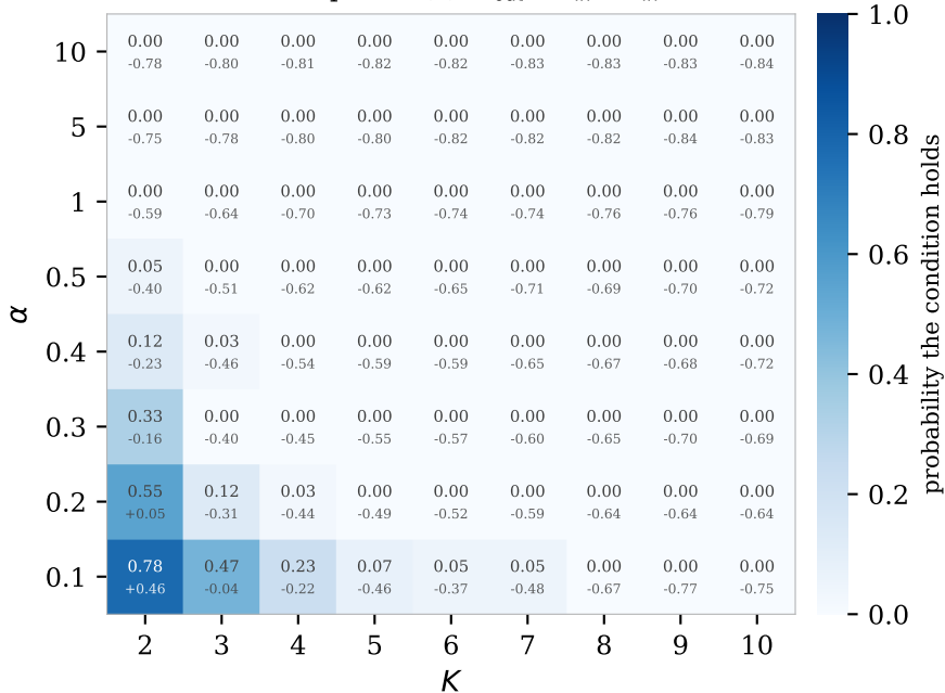
Assumption 4(a): \Delta_{\text{out}} - \Delta_{\text{in}} > \Delta_{\text{in}}
