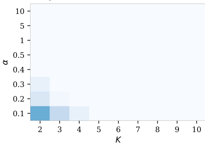
Assumption 5 (balance): \Delta_{\text{out}} - \Delta_{\text{in}} > (w_{\text{max}}/w_{\text{min}}) \Delta_{\text{in}}
