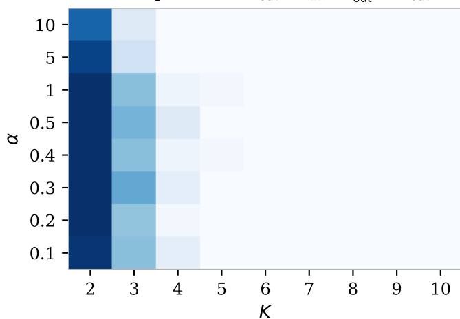
Assumption 4(b): \Delta_{\text{out}} - \Delta_{\text{in}} > \Delta_{\text{out}}^{\text{max}} - \Delta_{\text{out}}
