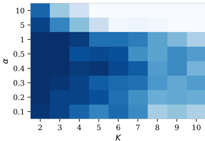
Assumption 3 (separation): \Delta_{\text{out}} > \Delta_{\text{in}}
