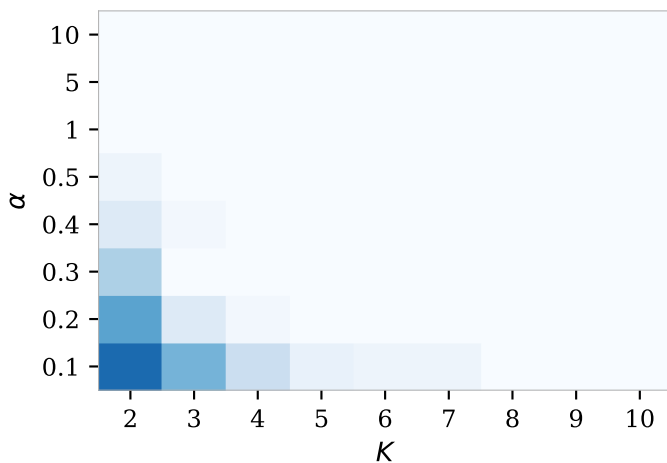
Assumption 4(a): \Delta_{\text{out}} - \Delta_{\text{in}} > \Delta_{\text{in}}
