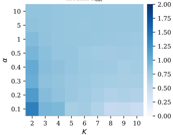
median \Delta_{\text{out}}
