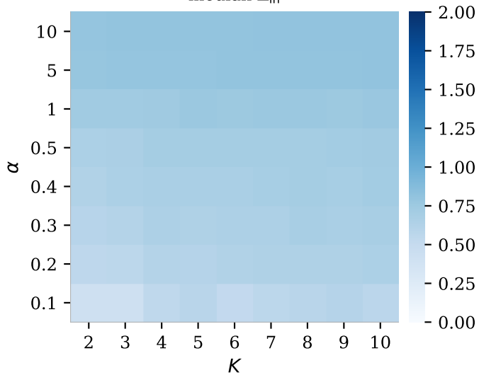
median \Delta_{\text{in}}
