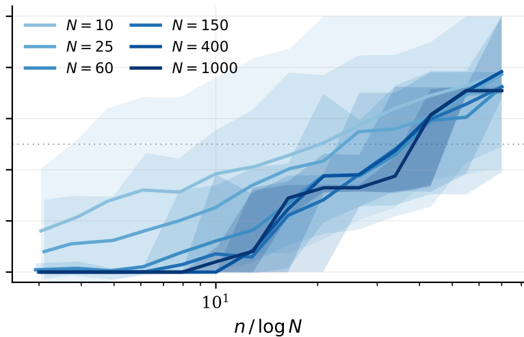
rescaled horizon \lambda = n/\log N
