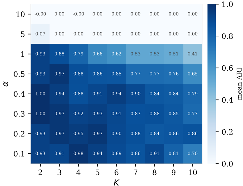
mean ARI at n = 800
