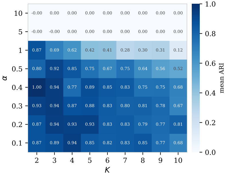
mean ARI at n = 400
