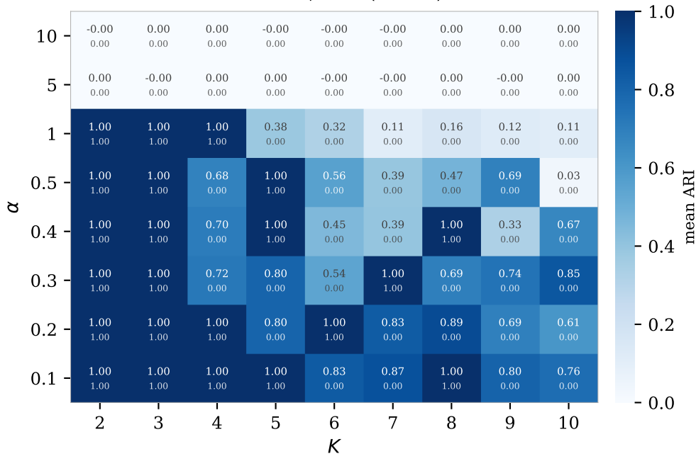
single linkage, n = 300 , N = 300 mean ARI, and \hat{P}(\text{ARI} = 1)
