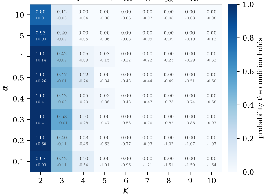
Assumption 4(b): \Delta_{\text{out}} - \Delta_{\text{in}} > \Delta_{\text{out}}^{\text{max}} - \Delta_{\text{out}}
