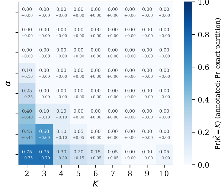
threshold of Theorem 3.9, M(\log N/n)^{1/4}
