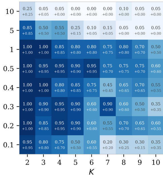
safeguarded profile rule
