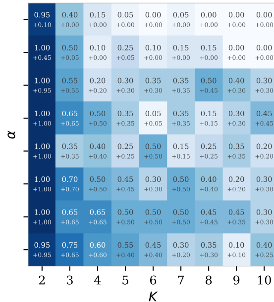
maximal silhouette width (PAM)
