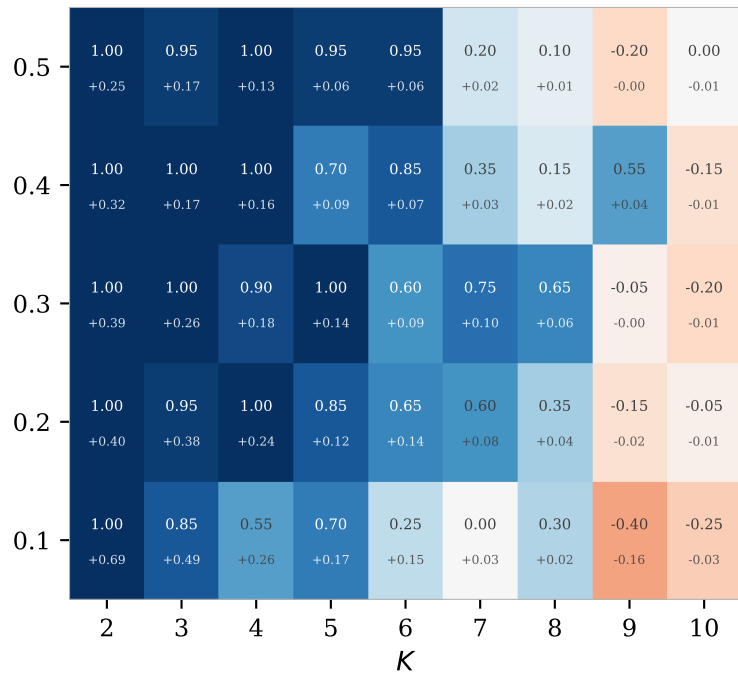
Markov chains
