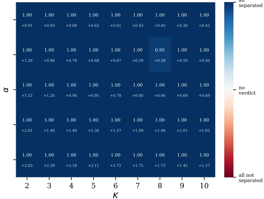
multichannel HMMs
