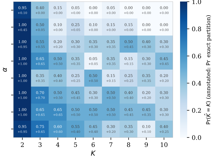
maximal silhouette width (PAM)
